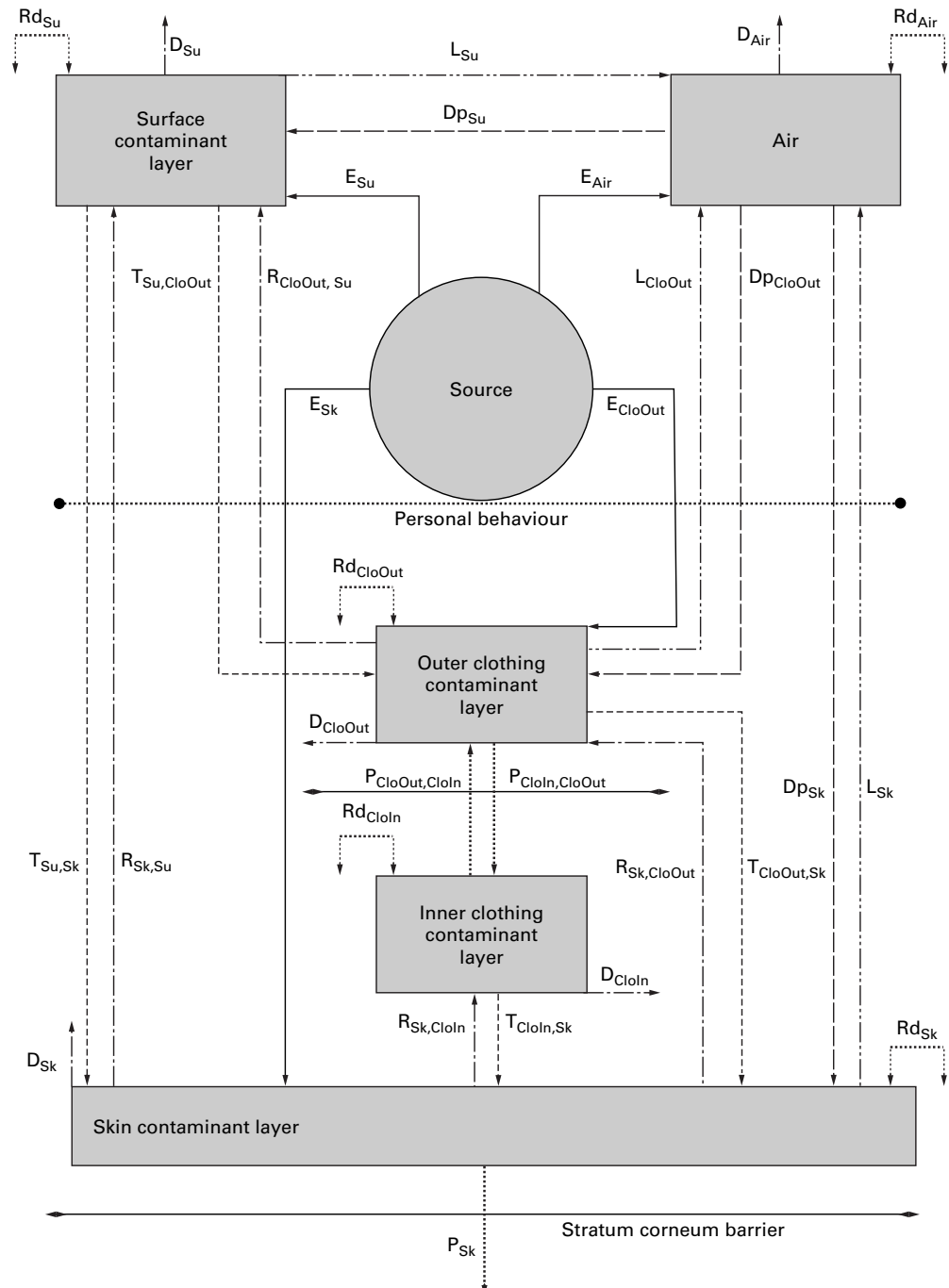
Overview of the conceptual model, compartments and rate constants. E =emission (—); Dp =deposition (---); L =resuspension or evaporation (-.-.-); T =transfer (.....); R =removal (----); Rd =redistribution (-----); D =decontamination (-.-.-.-); P =penetration and permeation (.....).
