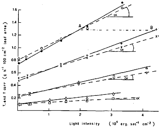
FIG. 7. The effect of light intensity ( \text{erg. sec}^{-1} \cdot \text{cm}^{-2} , fluorescent tubes) on the rate of transpiration of cut leaves of Hyoscyamus in potometers ( \text{g. h}^{-1} \cdot 100 \text{ cm}^{-2} leaf area) at various air temperatures and various relative humidities; \bullet — \bullet 29°C, 33% r.h.; + — + 24°C, 45% r.h.; \Delta — \Delta 15.2°C, 50% r.h.; \diamond — \diamond 5.2°C, 60% r.h. Broken lines with corresponding symbols the same, corrected for differences between leaf temperature and air temperature ( T_{\text{corr}} ).
