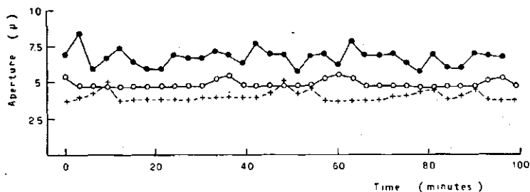
FIG. 20. Time course of variation in slit width in \mu of three stomata of a bean leaf at 21°C air temperature in continuous strong light ( 20 \times 10^4 \text{ erg. sec}^{-1} \text{ cm}^{-2} ) and normal air as observed by microscopy.
