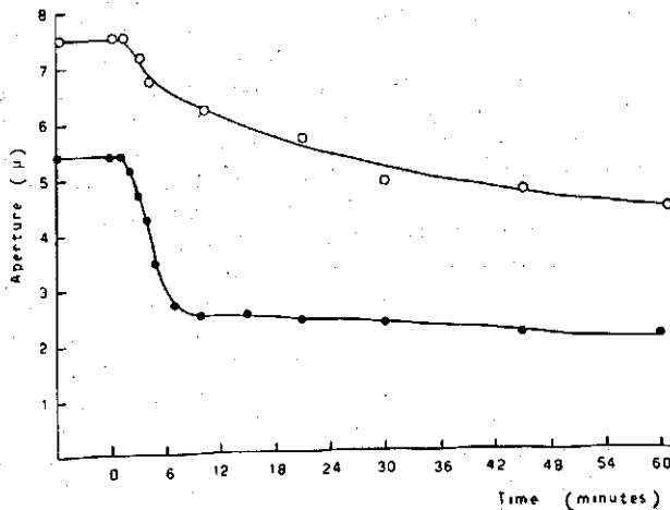
FIG. 16. Closing reaction of the stomata of bean leaves at 21 °C air temperature (slit width in μ, average of 30 as observed by microscopy). (●—●) upon shift from strong light (20 × 10 4 erg.sec -1 .cm -2 ) to weak light (4 × 10 4 erg.sec -1 .cm -2 ), in normal air; (○—○) same in CO 2 -free air.
