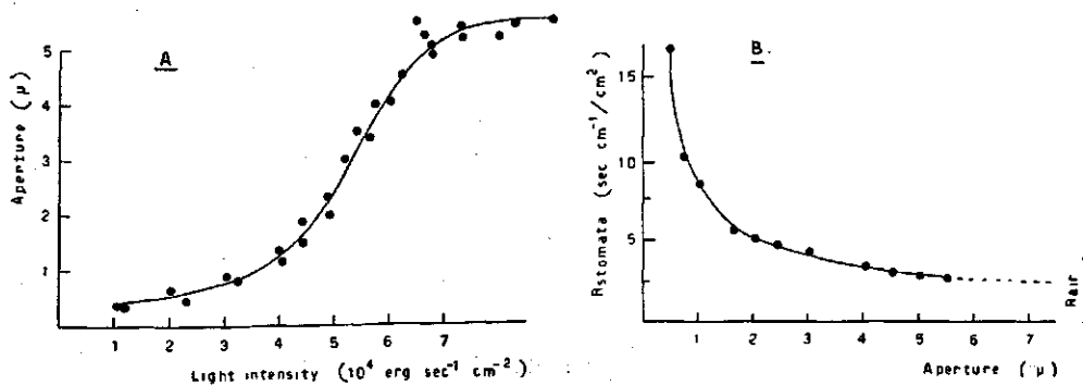
FIG. 14. A. Width of the stomatal slit (in \mu , average of 20 measurements) in relation to light intensity ( \text{erg}\cdot\text{sec}^{-1}\cdot\text{cm}^{-2} , mercury lamp); microscope observation, bean leaf.
