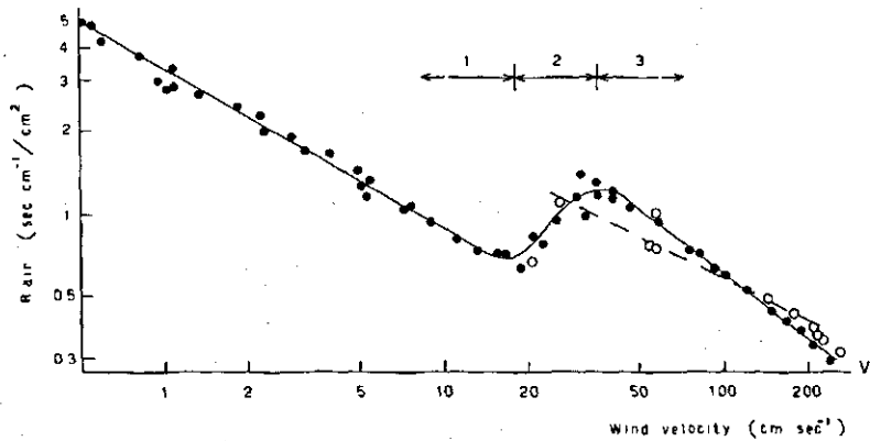
FIG. 5. The effect of wind velocity ( V , in \text{cm}\cdot\text{sec}^{-1} ) on the average resistance to water vapour transport of the boundary layer of air ( R_{air} , in \text{sec}\cdot\text{cm}^{-1} per \text{cm}^2 area); (1) laminar air movement, (2) semi-turbulent air movement, (3) turbulent air movement; (O—O), some data of MARTIN (1943) and his suggested curve.
