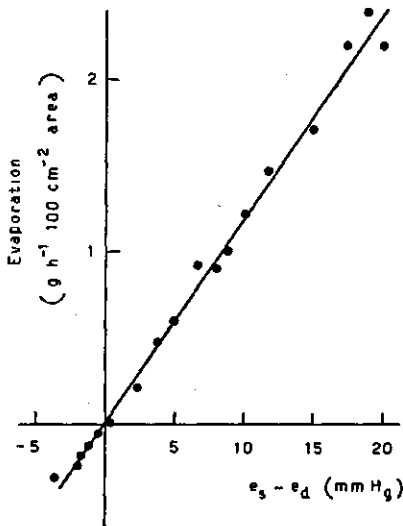
FIG. 3. Evaporation of a water surface ( \text{g.h}^{-1} \cdot 100 \text{ cm}^{-2} ) in relation to difference in saturation vapour pressure at surface temperature and actual vapour pressure of the air ( e_s - e_d , in mm Hg).
