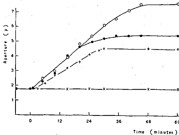
Fig. 15. Opening reaction of the stomata of bean leaves at 21^\circ\text{C} air temperature (slit width in \mu , average of 30 as observed by microscopy). (● — ●), upon shift from normal air (0.03% \text{CO}_2 ) and weak light ( 4 \times 10^4 \text{ erg. sec}^{-1}.\text{cm}^{-2} ) to normal air and strong light ( 20 \times 10^4 \text{ erg. sec}^{-1}.\text{cm}^{-2} ); (○ — ○), same for shift to \text{CO}_2 -free air and strong light, and (+ — +) for shift to \text{CO}_2 -free air and weak light; (× — ×), continued exposure to normal air and weak light.
