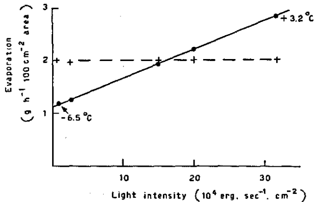
FIG. 4. Evaporation ( \text{g.h}^{-1} \cdot 100 \text{ cm}^{-2} ) and temperature of the evaporating water surface in relation to light intensity; (●—●) at 29.5^\circ\text{C} air temperature and 29% r.h.; (+—+) same, corrected for differences between surface temperature and air temperature; e_a - e_d = 22 \text{ mm Hg} .
