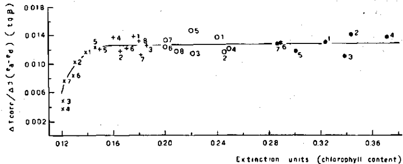
FIG. 13. The increase in transpiration of tomato leaves ( \text{g}\cdot\text{h}^{-1}\cdot(2.5 \times 10^6 \text{ stomata})^{-1} ) per unit increase of incident light intensity ( 10^4 \text{ erg}\cdot\text{sec}^{-1}\cdot\text{cm}^{-2} , sodium light), per unit vapour pressure difference ( \epsilon_a - \epsilon_d , in mm Hg) in relation to the chlorophyll content of the leaves, expressed as extinction value at 665 \text{m}\mu (cf also fig. 12). Symbols represent the light conditions in which the experimental plants were grown and the age of the leaves.
