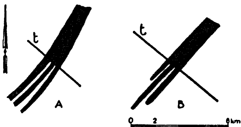
FIG. 56. Outline of the ramifications of the beach-banks near Lisse (A) and Noordwijk (B). t: tangent at the points of ramification.
