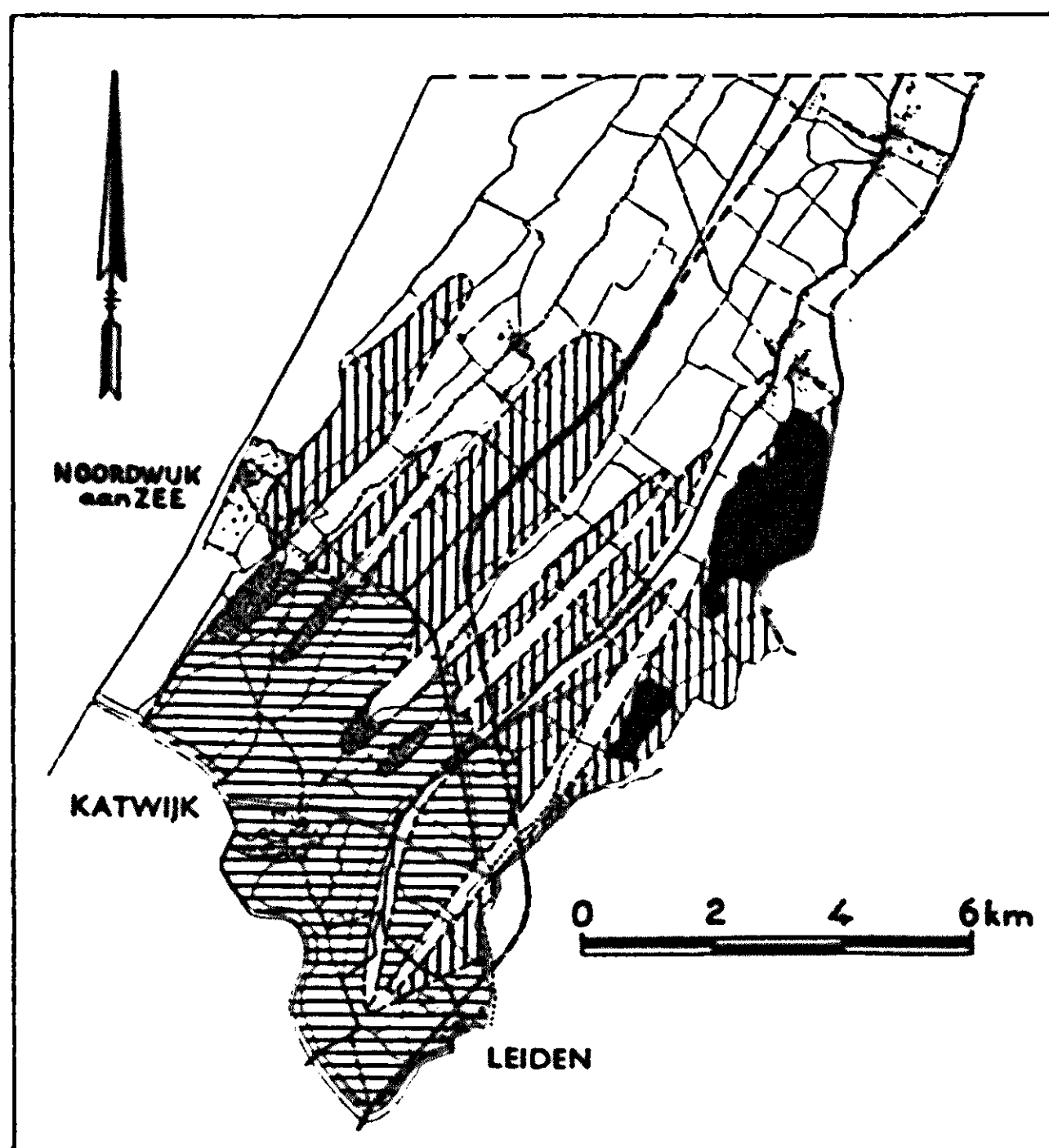
FIG. 11. General view of the situation of the beach-plain sand soils.
