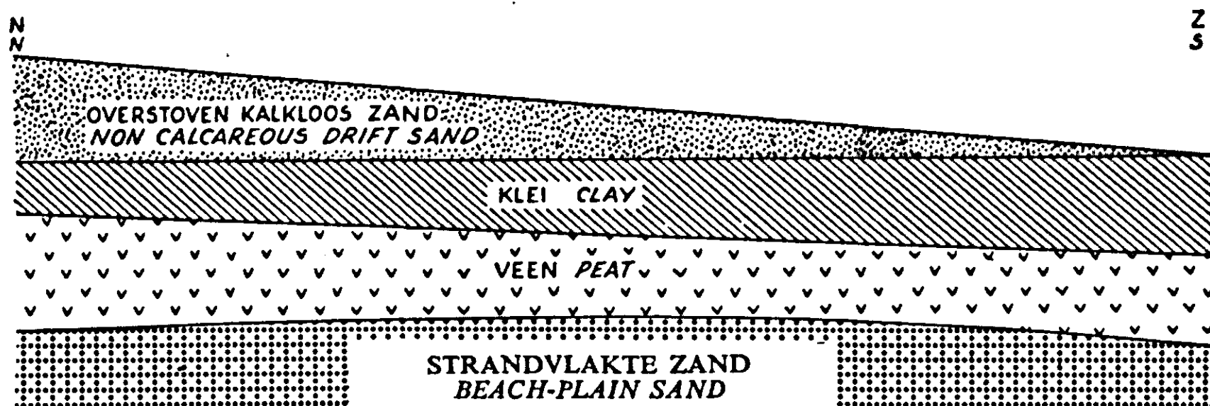
FIG. 41. Longitudinal section of the transition from beach-plain soils to estuary soils.
