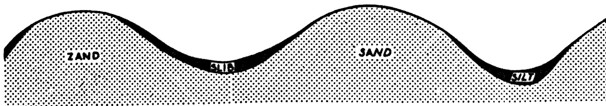
FIG. 7. Longitudinal section of a low spur of the beach-bank near Noordwijk. In low places silt has been deposited under marine conditions.
