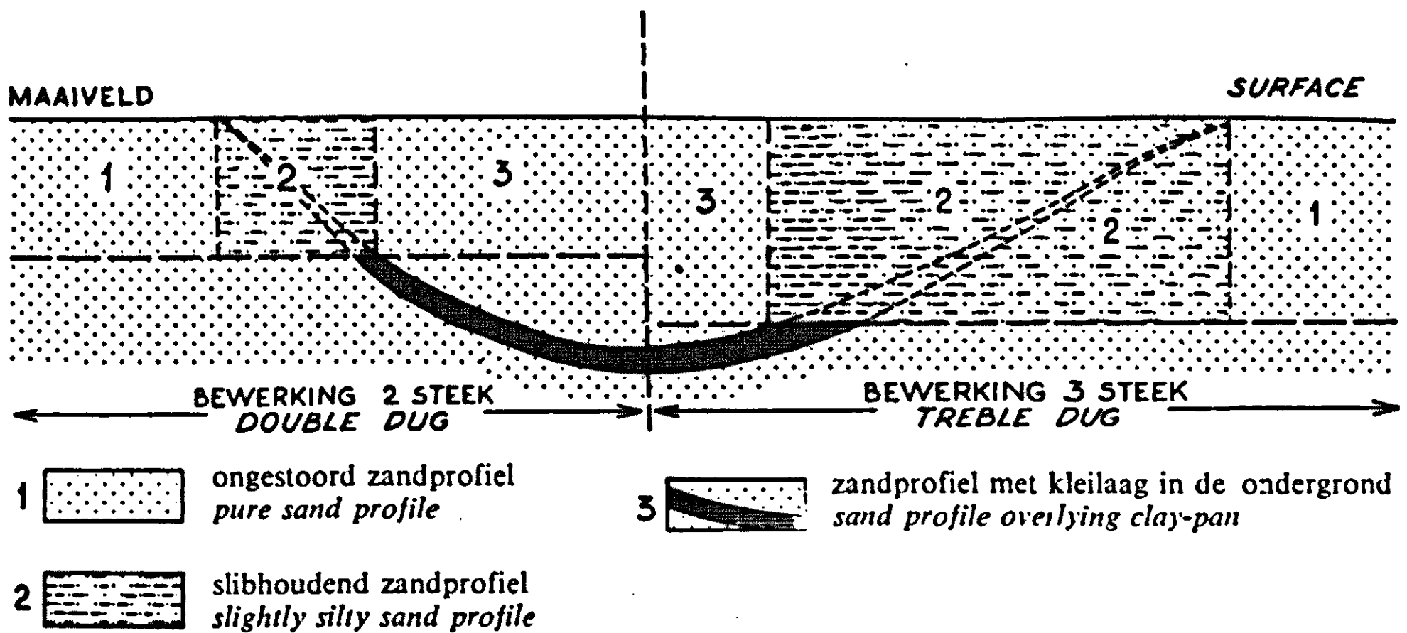
FIG. 9. Effect of digging in a profile with a shallow clay pan.
