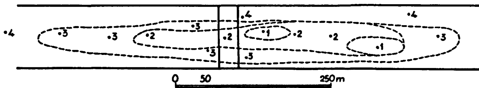
FIG. 29. Slope of the calcareous sand along the beach-bank of Noordwijkerhout. From the outcrops of calcareous sand the depth at which chalk is found gradually increases.
