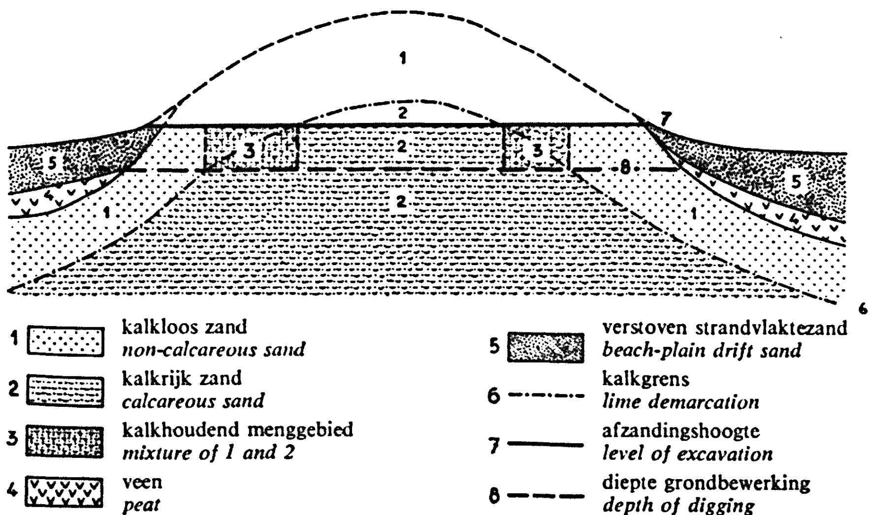
FIG. 3. Cross section of a beach-bank showing in the centre a rise of the demarcation line between calcareous and non-calcareous sand above the level of excavation.
