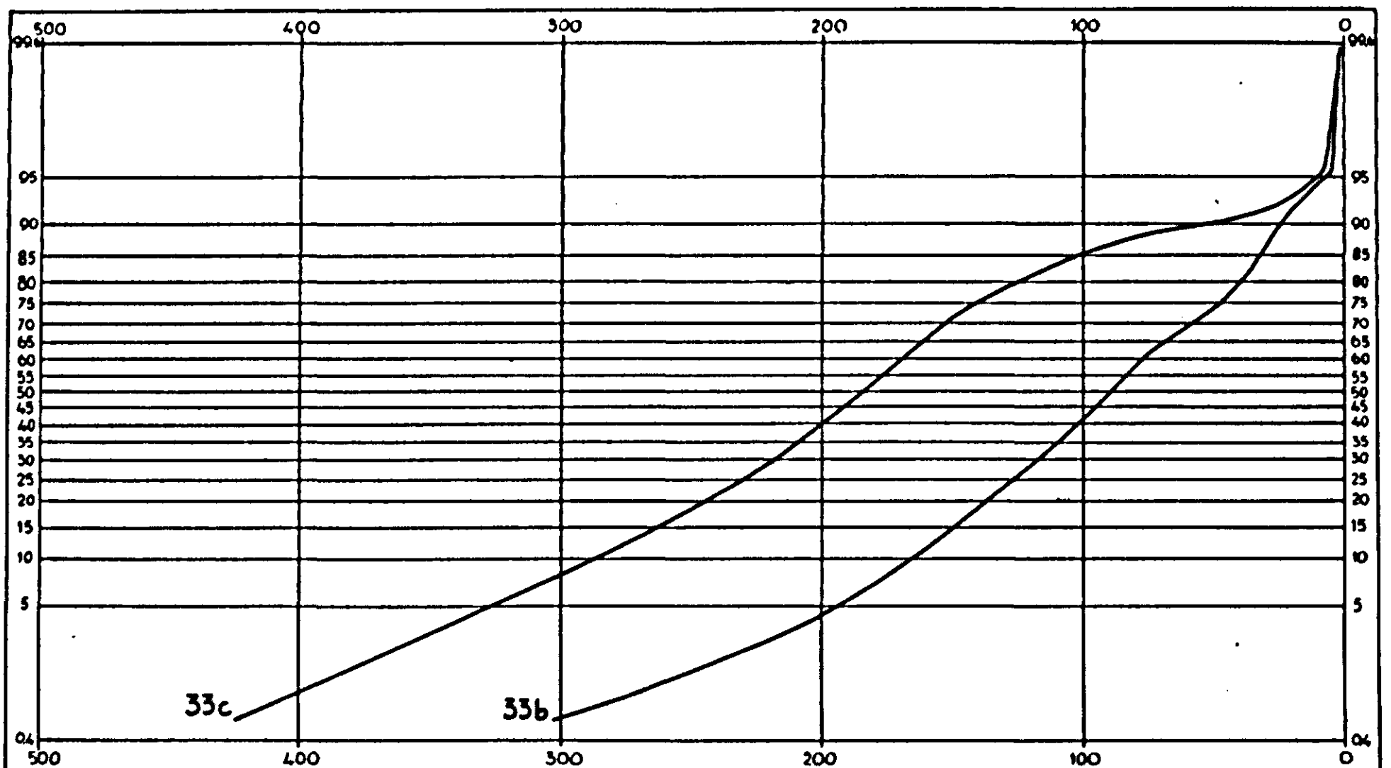
FIG. 73. Summation curves of a silty sandy „gors”-soil (33b) and a slightly silty beach-bank soil (33c). Except in mechanical composition the soils also differ in calcium content: the „gors”-soil is calcareous, the beach-bank soil is non-calcareous. Compare with fig. 74 a and b.
