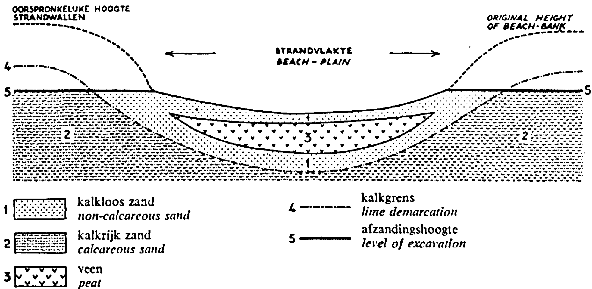
FIG. 11. General view of the situation of the beach-plain sand soils.
