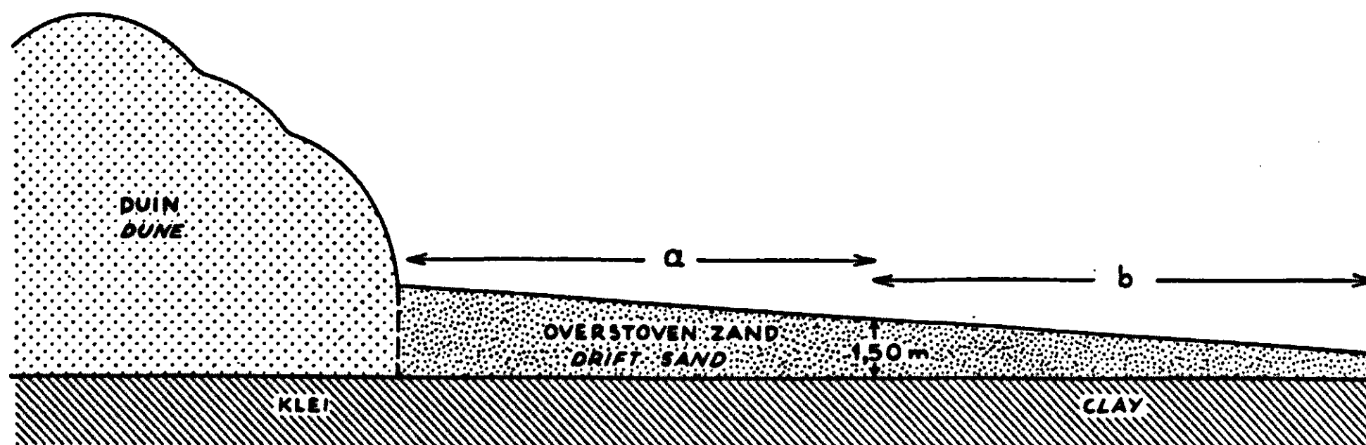
FIG. 22. Situation of a drift-sand cap on the inner slope of a dune. a. clay layer not reached by auger; b. clay layer reached by auger.
