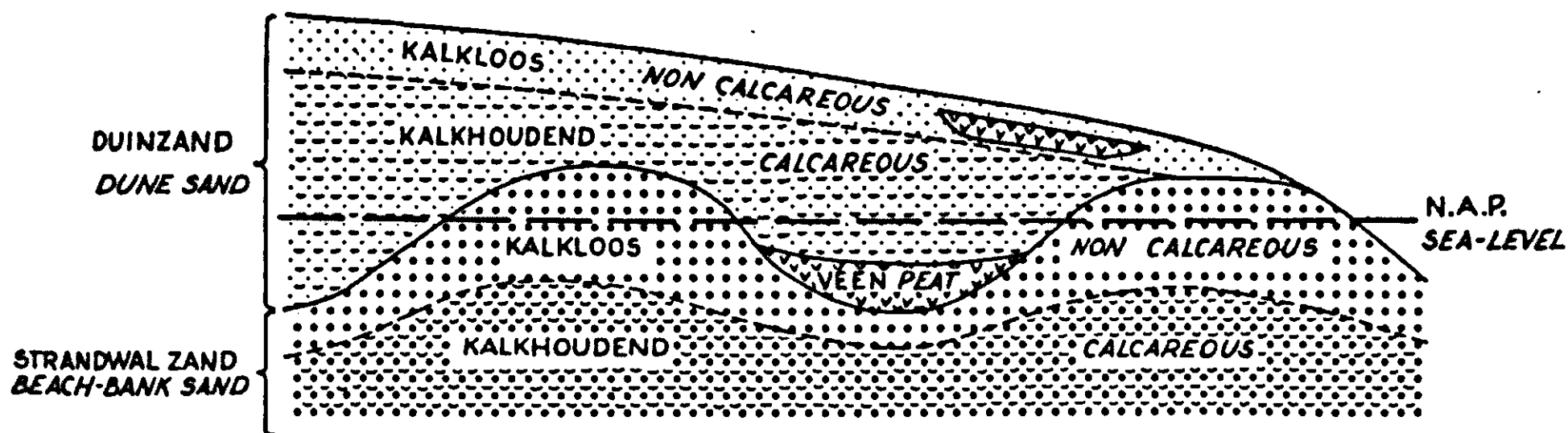
FIG. 53. Cross section west-east showing the wind drift dune-sand cap overlying the beach-bank landscape.
