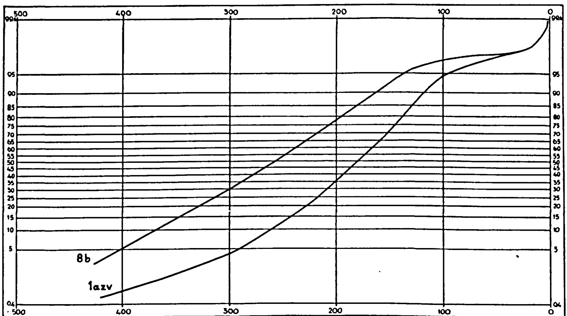
FIG. 65. Summation curves of a normal sediment (8b) and a calcareous beach-bank sand (1azv).
