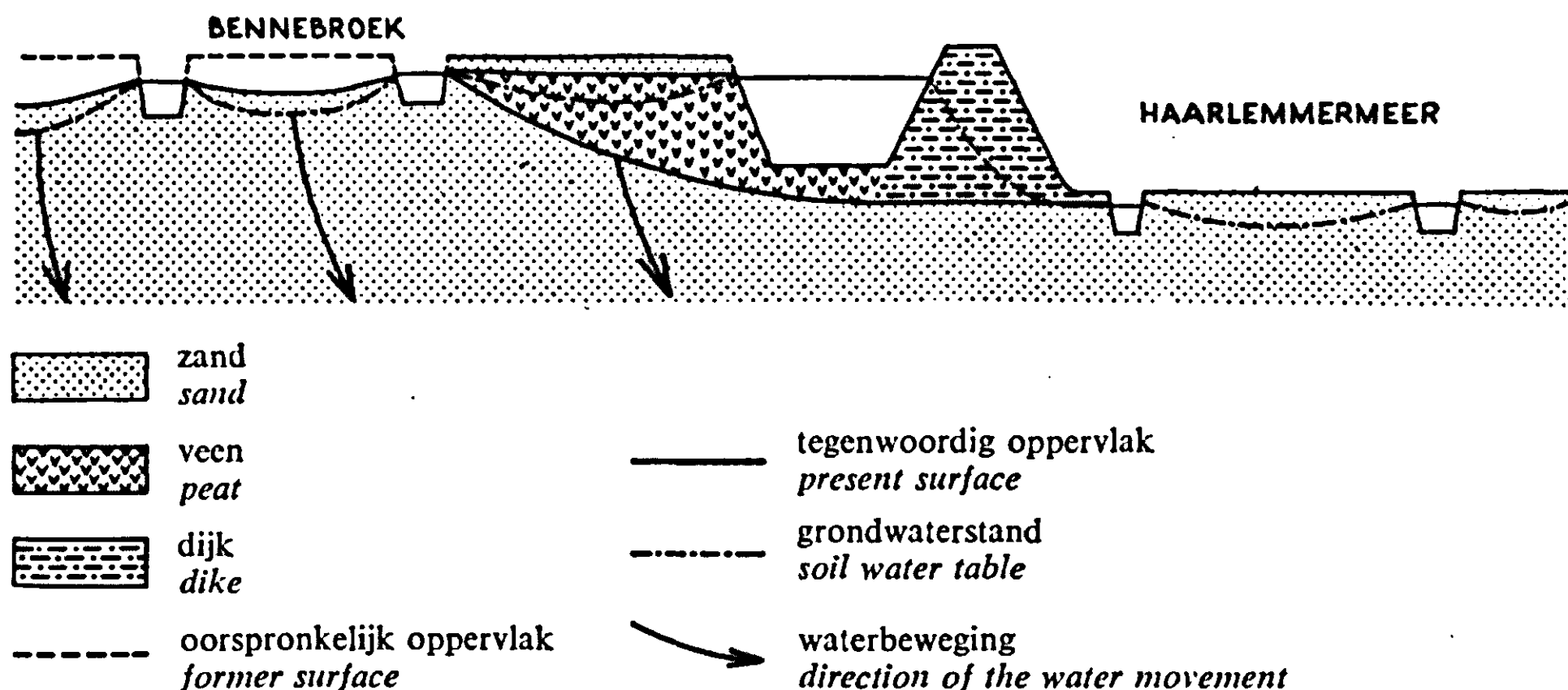
FIG. 50. Outline of a hydrological cross section from Bennebroek to the Haarlemmermeer.
