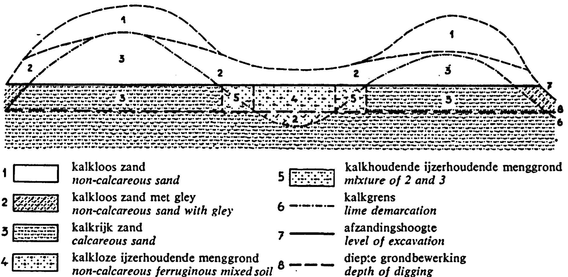
FIG. 5. Cross section of two beach-banks near the point of ramification. In the depression between the banks the soil is rich in iron.
