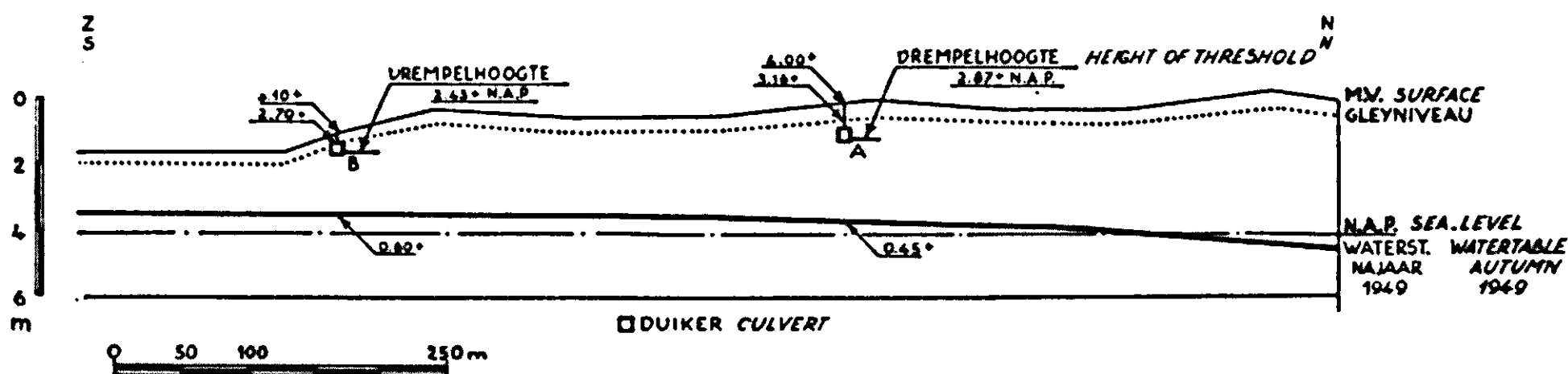
FIG. 40. Section north-south of the Langeveld indicating the former watertable (gleyniveau) and the watertable in 1949.
