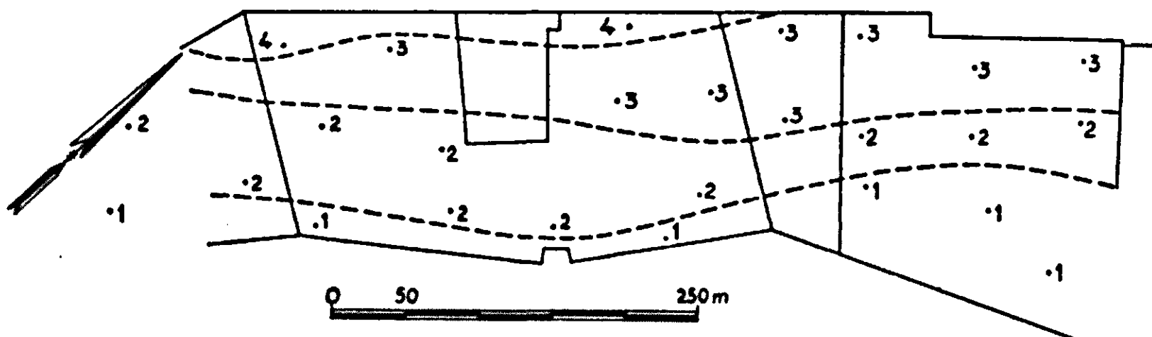
FIG. 28. Lateral dispersion of the calcareous sand in the beach-bank of Noordwijkerhout. Towards the beach-bank the depth at which the calcareous sand occurs increases.
