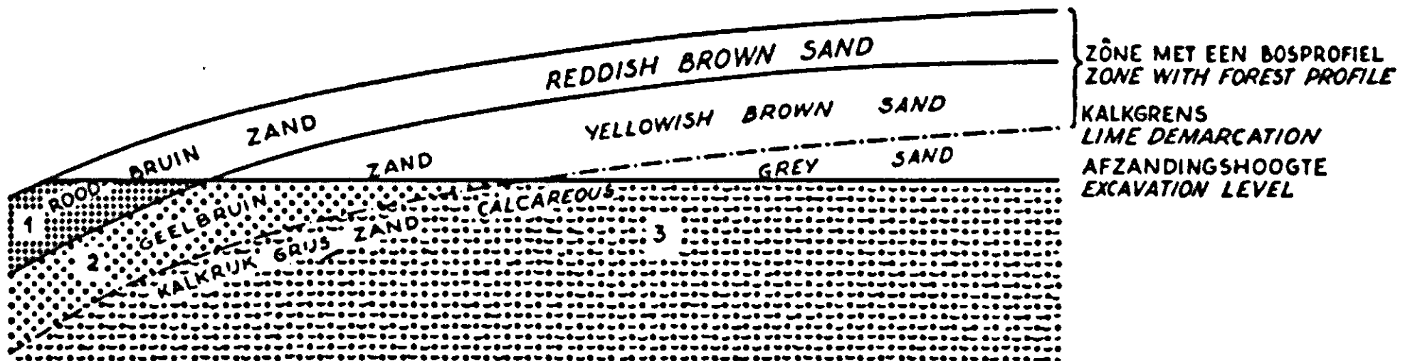
FIG. 16. Longitudinal section of a beach-bank with an indication of the influence of a forest profile.
