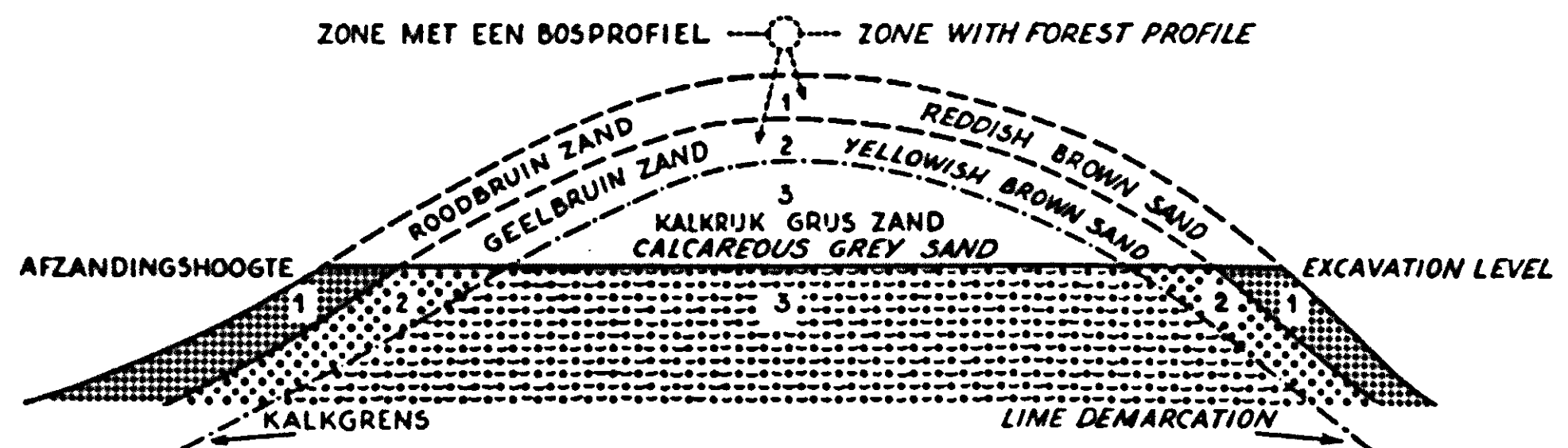
FIG. 17. Cross section of a beach-bank with an indication of the influence of the forest profile.
