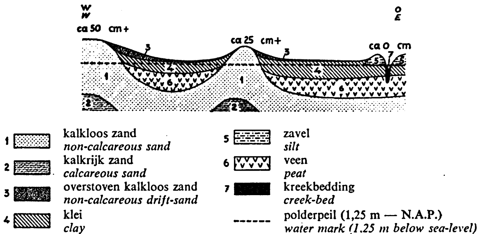
FIG. 42. Cross section of the Elsgeesterpolder from the ramification of the tidal gully to the west.
