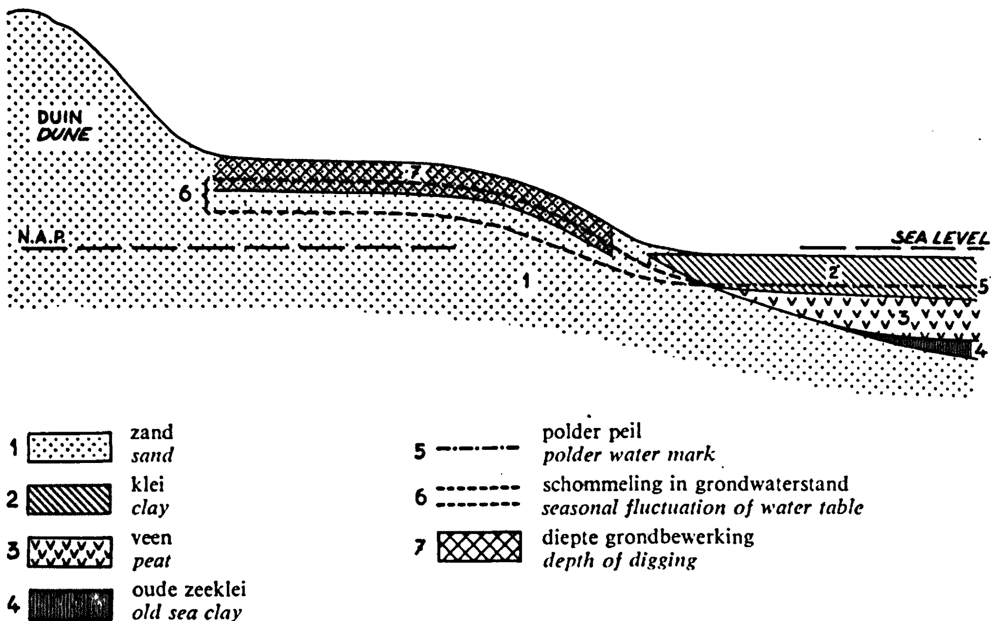
FIG. 44. Cross section east-west of the area north of Santpoort.
