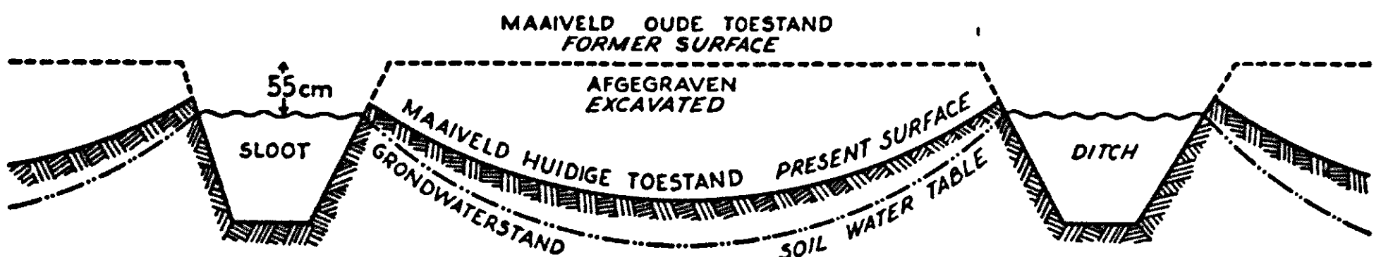
FIG. 49. Adaptation of the land surface to the lowered soil watertable on the bulb-farms near Bennebroek.
