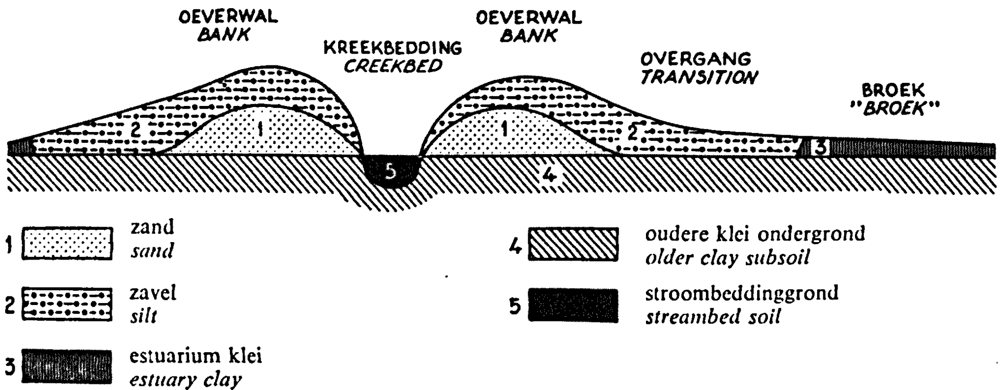
FIG. 13. Outline of the relative situation of the estuary soils.
