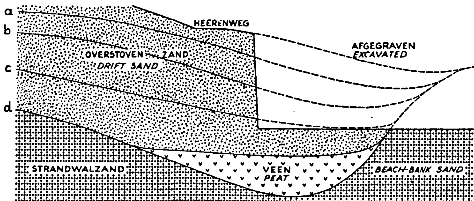
FIG. 32. Outline of a cross section of the beach-bank north of Noordwijkerhout. Numerous vegetation zones are noticeable some which could be dated from archaeological finds.
