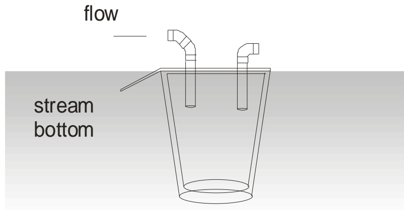
Figure 4. Scheme of the mineral and organic material collector.
