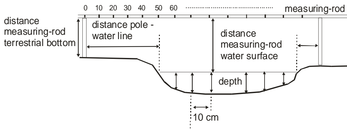
Figure 3. Scheme to measure a depth profile using a measuring-rod along fixed poles.
