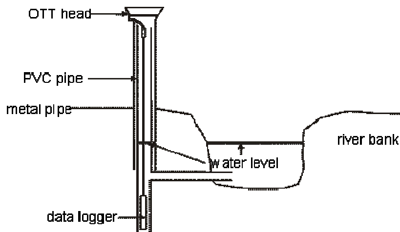
Figure 1. Water level measurement.
