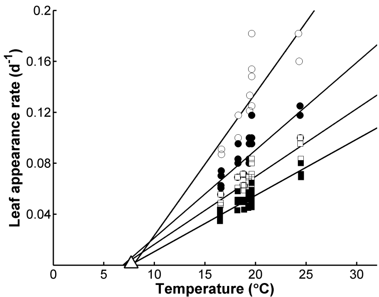
Fig. A1.5.9: Base temperature T_b (open triangle) estimated on basis of time -1 to appearance for leaf 2 (open circles); leaf 3 (closed circles); leaf 4 (open squares) and leaf 5 (closed squares) of cultivar Ayana plotted against the temperatures: 16.3, 18.3, 18.8, 19.3, 19.8 and 24.3 °C. Lines represent simple linear regression lines used to extrapolate to a rate of zero, where T_b = 7.8^{\circ}\text{C}
