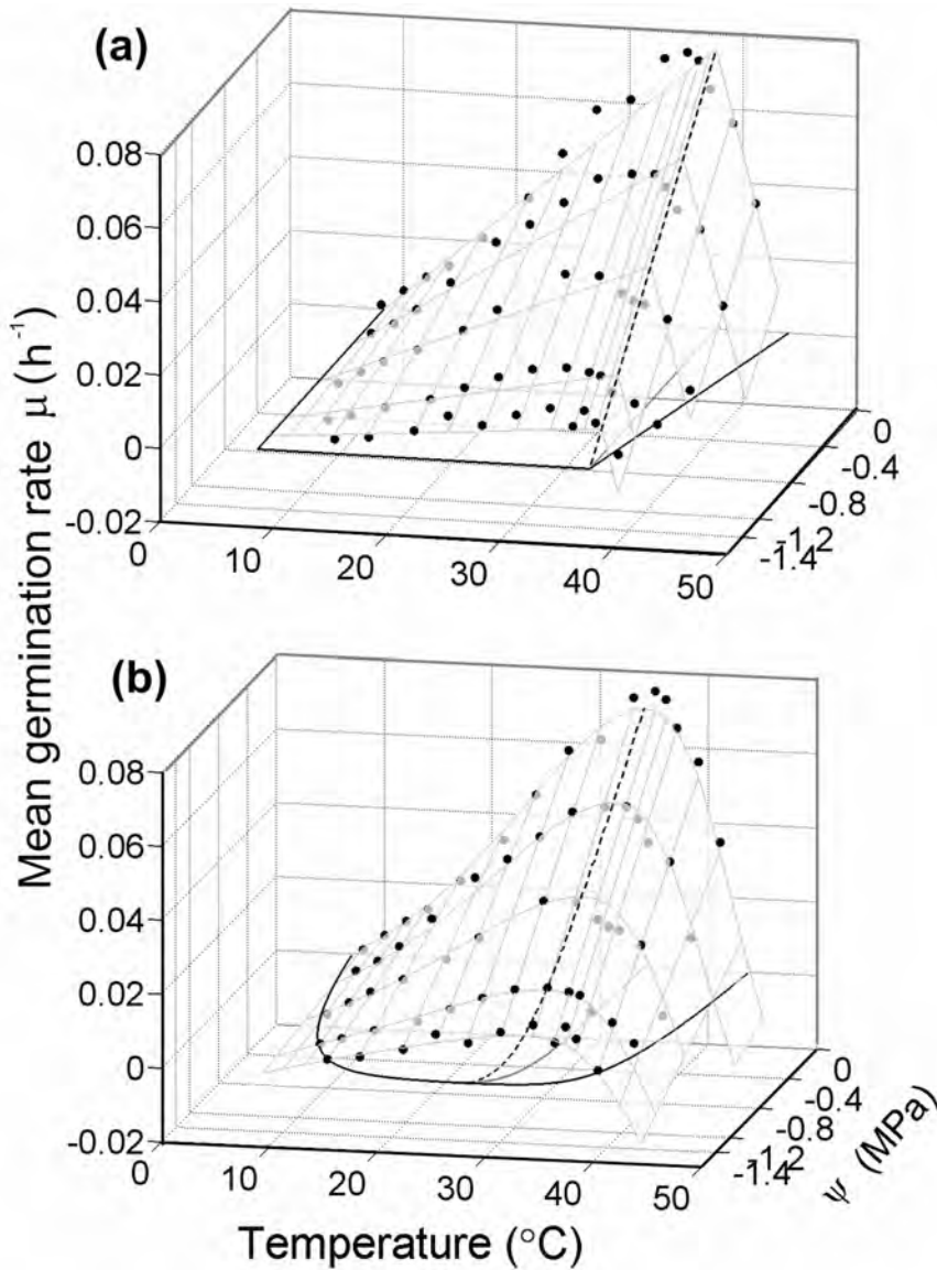
Fig. 2.4: Mean germination rate ( \mu ) (dots) (z-axis; \text{h}^{-1} ) as a function of water potential ( \psi ) (x-axis; MPa) and temperature ( T ) (y-axis; ^{\circ}\text{C} ) for (a) the HTT model (eqn 2.1) and (b) the HTR model (eqn 2.4, 2.7 and 2.8). The gridded surface represents the modelled response surface. Black dots are above the surface whereas grey dots are below it. The U-shaped solid black line is the intersection between the response surface and the plane defined by \mu = 0 . This U-shaped solid black line represents the relationship between base water potential and temperature ( \psi_b(T) ). The same U-shaped solid black line shows cardinal temperatures T_b(\psi) and T_c(\psi) as a function of water potential. The maximum germination rate at each water potential is represented by the broken black line. The corresponding optimum temperature T_o as a function of water potential ( \psi ) is represented by the solid grey line drawn at \psi = 0 in the ( T , \psi ) plane.
