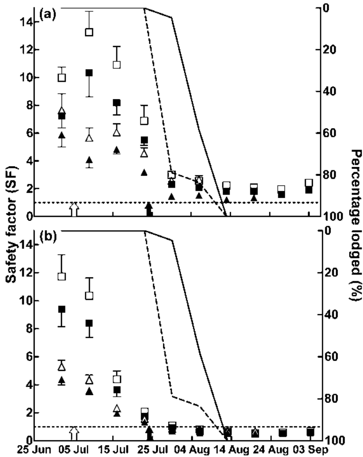
Fig. 3.7: Factor of safety (symbols) for (a) shoot ( SF_S ) and (b) root ( SF_R ), during the season; for cultivar Ayana wet (closed triangle) and dry (open triangle) and cultivar 04T19 wet (closed square) and dry (open square). Observed lodging percentage in unsupported fields for Ayana (broken line) and 04T19 (solid line). Horizontal dotted line is the critical safety factor ( SF=1 ). Flowering time defined as 50% flowering plants is shown for Ayana (open arrow) and 04T19 (closed arrow). Error bars indicate standard error ( n = 6 ) and when not visible fall within the symbol.
