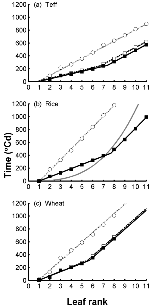
Fig. 5.1: Time required for a leaf to appear, in °Cd calculated with (T - T_b) \cdot p ((a) for teff T_b = 7.8 °C, (b) for rice T_b = 10 °C and (c) for wheat T_b = 0 °C), plotted against leaf rank counted acropetally. Data points of each species represent leaf appearance data from a single representative main stem. Data points represented by closed squares are based on air temperature and are described with eqn 5.1a and 5.1b (solid line); open squares represent time required on basis of both soil and later air temperature (broken line eqn 5.1a and 5.1b); open circles are equal to the closed squares under the assumption that the second phyllochron, i.e. experiencing air temperature, is the representative pace of leaf appearance (dotted line calculated using eqn 5.5). The temperature required to lift the data points of the first phyllochron to the dotted line is the theoretical difference between air and soil temperature, T_\Delta . The grey line in (b) is the model y = x^b from Yin and Kropf (1996), expressing time in days in contrast to degree days as in the original publication.
