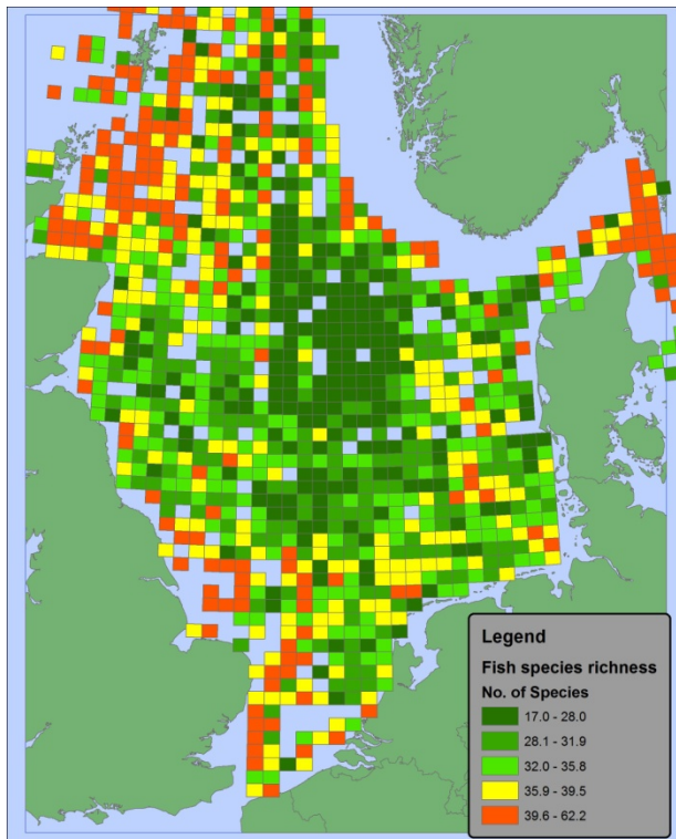
Figure 11 Spatial pattern of fish species richness in relation to percentage area available to OWP: greens = 75%, yellow = 50%, orange = 25%
