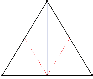
Figure 2a. BLE. Bisect the Longest Edge.
