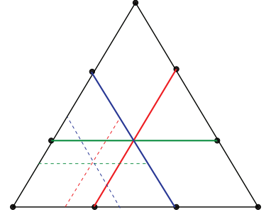
Figure 4c. ROD. Regular Overlapping Division.
