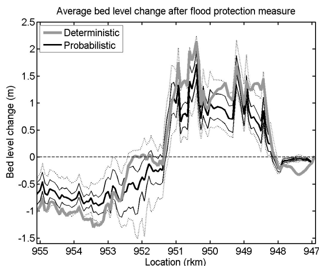
Figure 7. Differences in width-averaged bed level changes along the river axis (reference situation vs. flood protection measure).
