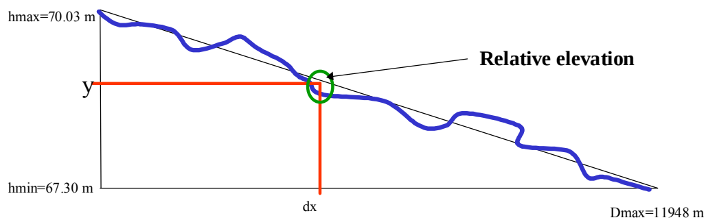
Figure 5. Representative diagram of slope calculation from the Digital Elevation Model (DEM) described in Smith et al. (2006), in order to obtain raster map values of relative elevation.
