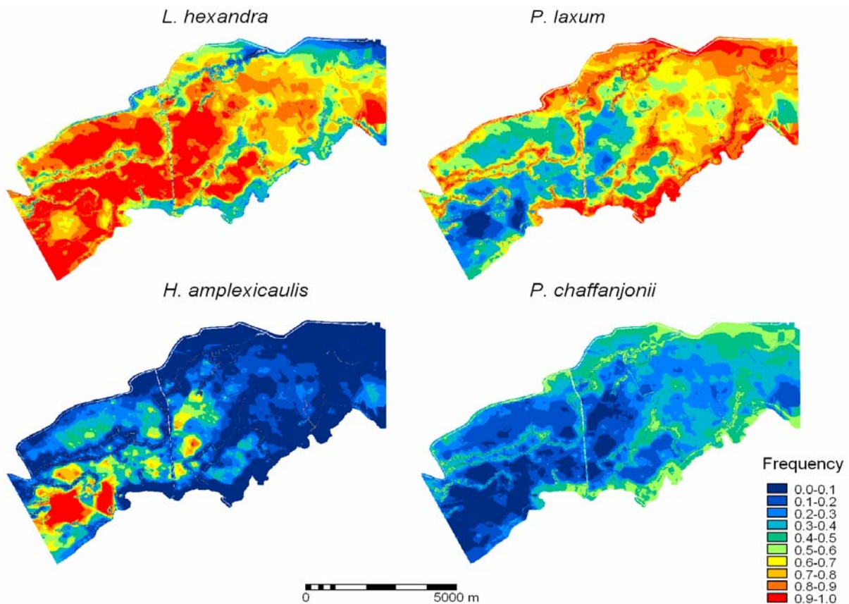
Figure 9. Model of species distribution of P. laxum , L. hexandra , H. amplexicaulis and P. chaffanjonii for frequency data based on Relative Elevation Model (RAM) in the flooding savanna of El Frio Biological Station, Venezuela.
