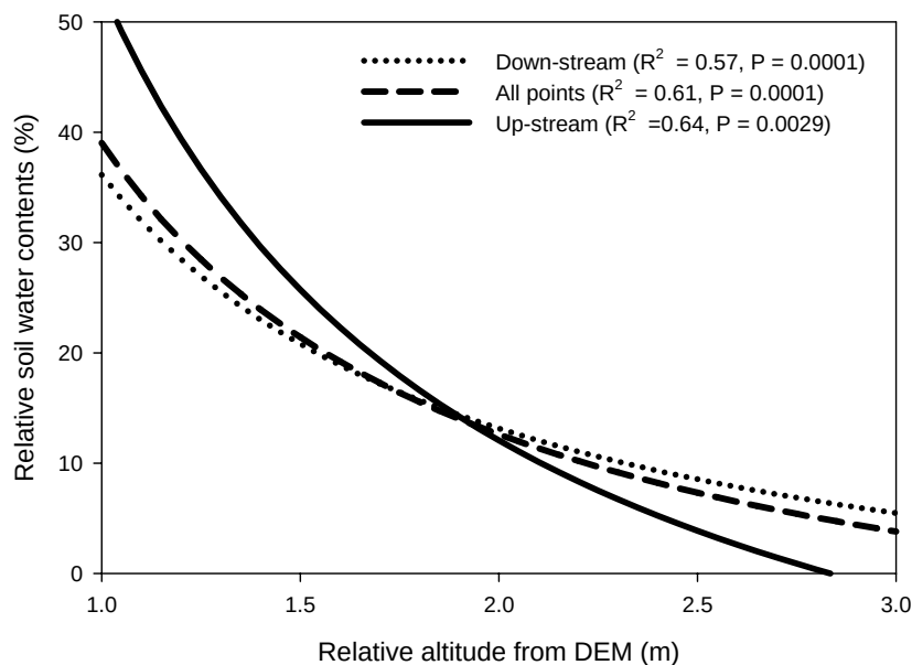
Figure 11. Regression curves between Relative Elevation Model values (RAM) derived from DEM (Smith et al. 2006) and Relative Soil Water Content values measured in the study area of the flooding savanna of El Frío Biological Station, Venezuela. Three sets of data were considered: all field observations, down stream of dike observations, and up-stream observations. Regression coefficients and significance values are indicated.
