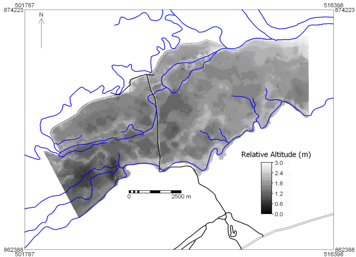
Figure 8. Relative Elevation Model (RAM) of the El Frío Biological Station study area, in the flooding savanna, Venezuela, derived from DEM (Smith et al. , 2006 and slope equation described in figure 5).
