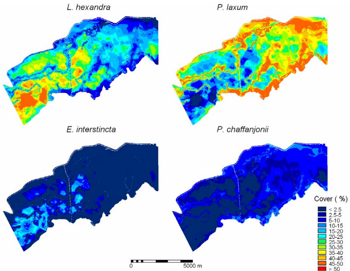
Figure 10. Model of species distribution of P. laxum , L. hexandra , E. interstincta and P. chaffanjonii for cover data based on the Relative Elevation Model (RAM) of the flooding savanna of El Frio Biological Station, Venezuela.
