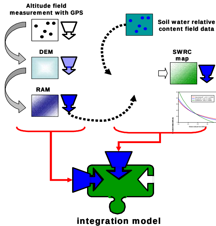
Figure 4. Scheme of the elaboration of the spatially explicit integrated model. Digital Elevation Model (DEM) derived from GPS measurements, and relative elevation model (RAM) derived from DEM. Relative soil water content (SWRC) map derived from regression between field data of relative soil water content and relative elevation model.
