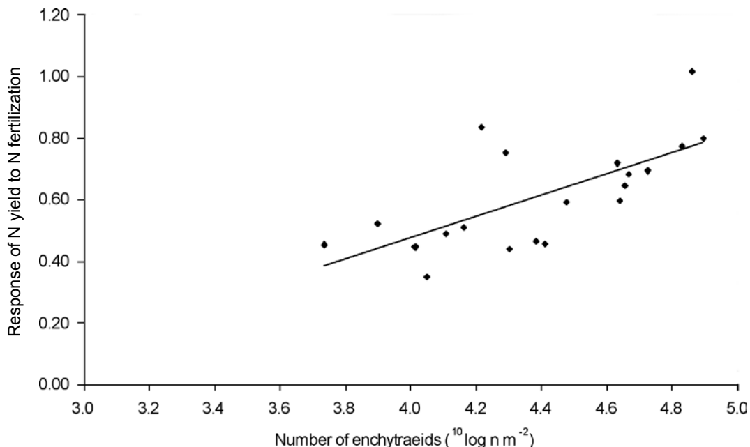
Fig. 7.4 Linear regression between total number of enchytraeids ( 10 \log n \text{ m}^{-2} ) and response of N yield to N fertilization ( R^2=0.47 , cross validated R^2=0.36 , P=0.047 ).
