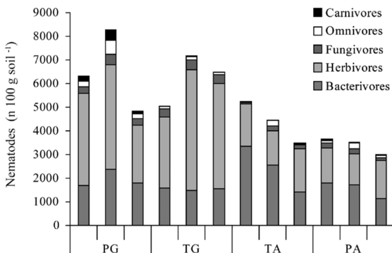
Fig. 2.3 Nematode abundance (n 100 g soil -1 ) divided over the different feeding groups in permanent grassland (PG), temporary grassland (TG), temporary arable land (TA) and permanent arable land (PA).
