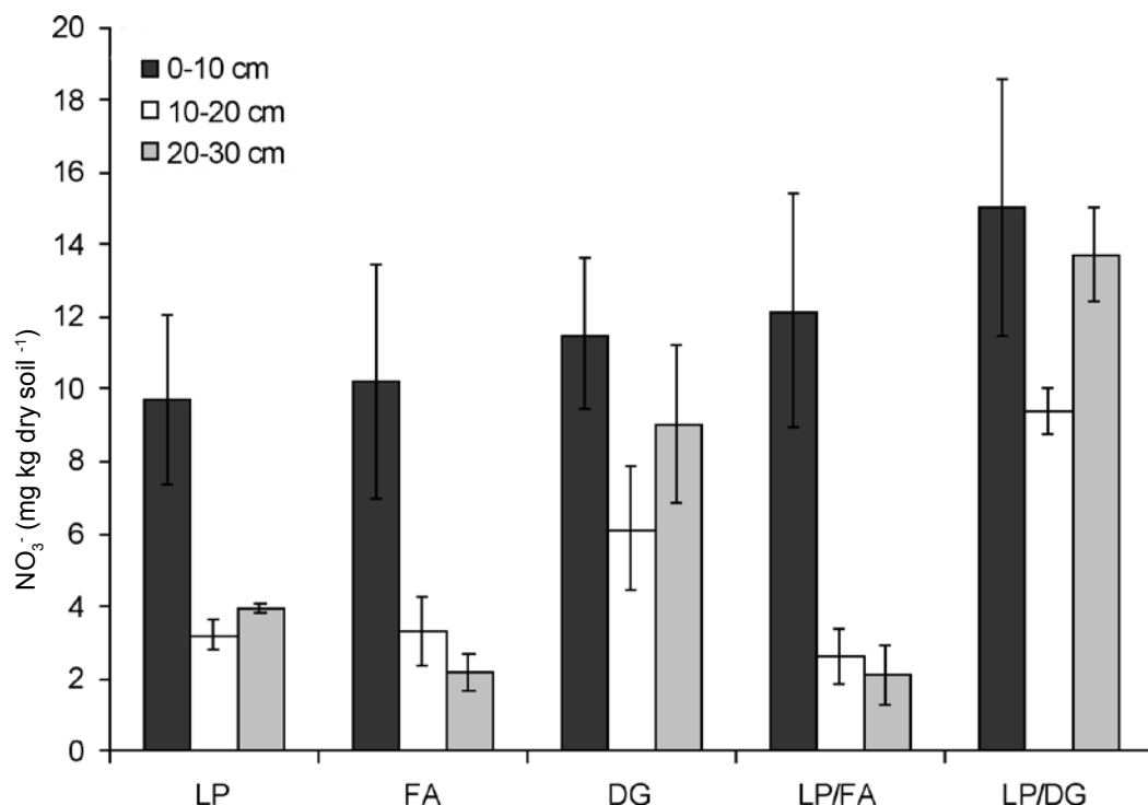
Figure 6.1 \text{NO}_3^- in grassland with Lolium perenne (LP), Festuca arundinacea (FA), Dactylis Glomerata (DG), a mixture of L. perenne and F. arundinacea (LP/FA), and a mixture of L. perenne and D. glomerata (LP/DG) at three soil depths (0-10 cm, 10-20 cm, 20-30 cm).
