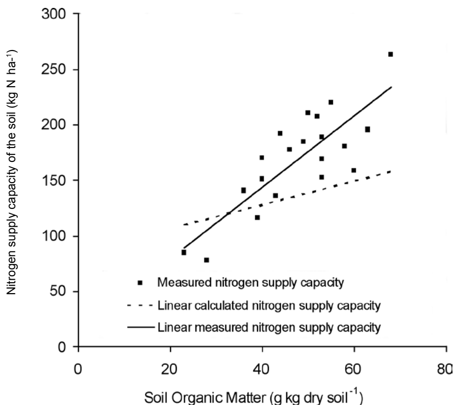
Fig. 7.3 Measured nitrogen supply capacity (N yield intercept) ( \text{kg N ha}^{-1} ) plotted against SOM ( \text{g kg dry soil}^{-1} ) and its linear regression ( R^2=0.67 , cross-validated R^2=0.59 , P<0.001 ), compared with the nitrogen supply capacity of the soil calculated from total N according to the Dutch grassland fertilization recommendation (section 7.2.6, http://www.bemestingsadvies.nl ).
