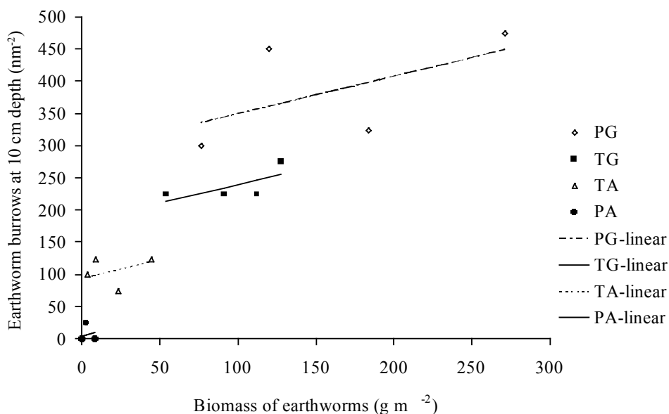
Fig. 2.2 Relation between earthworm biomass (g m -2 ) and earthworm burrows at 10 cm depth (n m -2 ) in 2004 for the four treatments ( R^2=0.93 ). Earthworm burrows (n m -2 at 10 cm depth) = treatment ( P<0.001 ) (intercept 5 for PA, 95 for TA, 182 for TG, 293 for PG) + 0.58 \times earthworm biomass (g m -2 ) ( P=0.044 ). Permanent grassland (PG), temporary grassland (TG), temporary arable land (TA), permanent arable land (PA).
