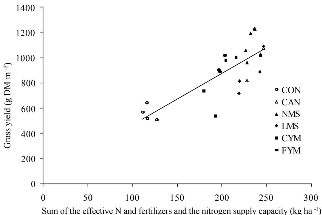
Fig. 4.2 Relationship between the sum of the effective N from the fertilizers ( \text{kg ha}^{-1} ) and the N supply capacity of the soil, and the dry matter yield of grass ( \text{g DM m}^{-2} ) ( R^2=63 , P<0.001 ). Treatments: unfertilized (CON) or fertilized with inorganic N fertilizer (calcium ammonium nitrate 27%, CAN), “normal” cattle manure slurry (NMS), manure slurry of cattle fed a ration low in protein (LMS), manure slurry mixed and composted with hay from roadsides (CYM) and farmyard manure from a deep-litter stable with dairy cows (FYM).
