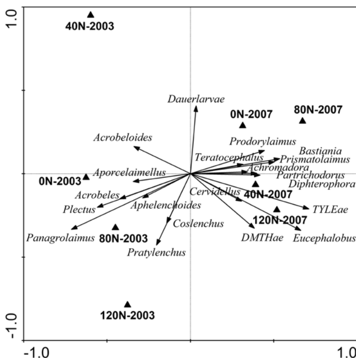
Fig. 5.1 Ordination diagram of the nematode taxa based on RDA with the model year (2003, 2007) x nitrogen application rate (0, 40, 80, and 120 kg N-total ha -1 ). The diagram explains 80.2% of the variance in the fitted abundances of the full model. Only nematode taxa of which >10% of their variance was explained by the axes 1 and 2 were plotted. Abbreviations of taxa: TYLEae, Tylenchidae; DMTHae, Dorylaimoidae + Thorneleminatae. The eigenvalues of axis 1 and 2 are 0.144 and 0.029, respectively.
