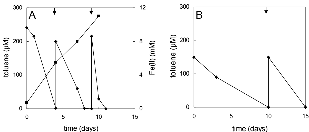
Figure 2. Toluene (♦) degradation coupled to the reduction of \text{Fe(III)NTA} (A; \text{Fe(II)} (■)) and \text{Mn(IV)O}_2 (B) by enrichments originated from Banisveld soil. Batch incubations performed in duplicate; both batches showed similar results, one batch is presented. Arrows indicate re-addition of toluene.
