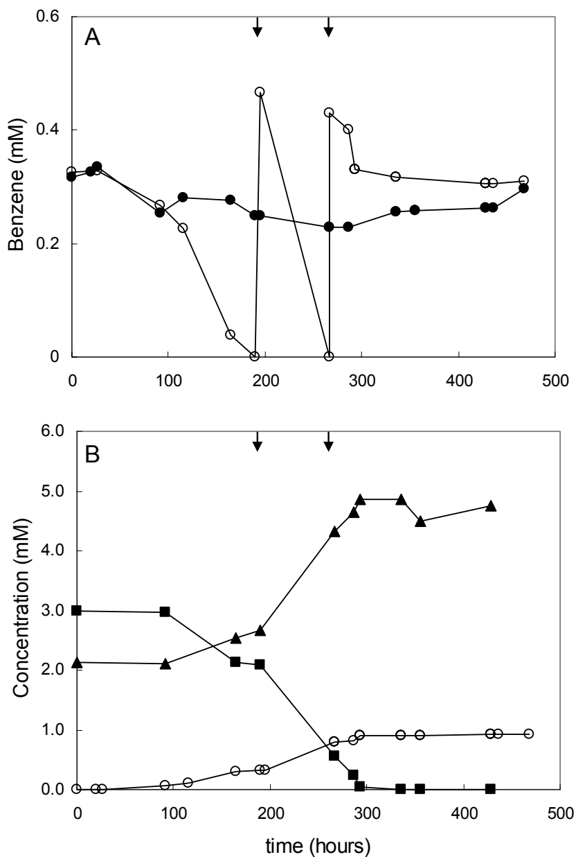
Figure 2. Mass balance of benzene biodegradation with chlorate as the electron acceptor. A: benzene (○) and sterile control (●) (average of two incubations; arrows indicate re-addition of benzene); B: cumulative amount of benzene degraded (○) and chlorate (■) and chloride (▲) measured (average of two incubations; arrow indicates re-addition of benzene).
