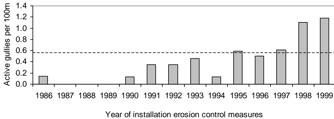
Figure 8.7. Virtual time series: erosion observed in 2000 in fields with erosion control measures installed between 1986 and 1999, compared with erosion in fields without erosion control (horizontal reference line y=0.58 ) in southern Mali (571 fields).
