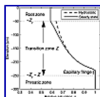
Figure 1. Idealized moisture profile. A root zone of fixed thickness Z_r and uniform relative moisture content s_r is connected to a phreatic zone by a transition zone with thickness Z .
