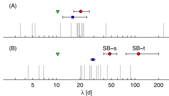
Figure 3. Distribution of \lambda for the GSWP-2 LSMs (vertical lines) at (a) Rheindahlen during the 1995 drought, and (b) SEBEX. Axis is logarithmic. Observations (circle) and GSWP-2 Multi-Model analysis (square) are both plotted with 95% confidence limits. Triangle indicates the Dardanelli et al. [2004] model.
