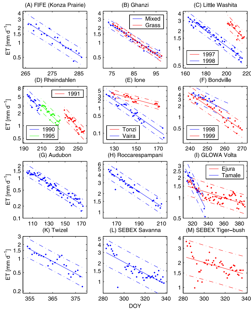
Figure 2. Daily ET versus day of year (DOY) for different sites under rainless conditions. Years and regression statistics are listed in Table 2. Note that the y -axis scale is logarithmic and that the scale of both axes can vary. Dashed lines correspond to the 95% prediction intervals.
