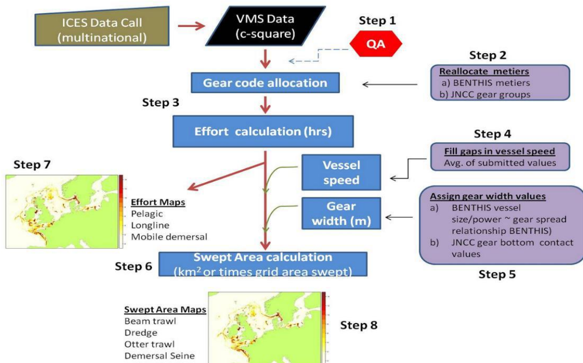
Figure 2.1. Workflow for the production of fishing intensity maps from aggregated VMS data (0.05° x 0.05° C-square resolution) (from ICES, 2016a). All métiers and vessel size/ gear spread relationships were derived from (Eigaard et al., 2016).
