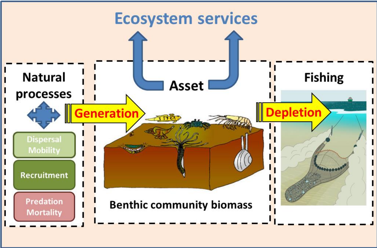
Figure 4.1 Basic processes determining the ecosystem asset, i.e. the biomass of the benthic invertebrate community, and how this asset is governed by processes contributing to its generation and recovery as well as by its depletion caused by fishing. The asset is mainly considered from its capacity to supply ecosystem services.
