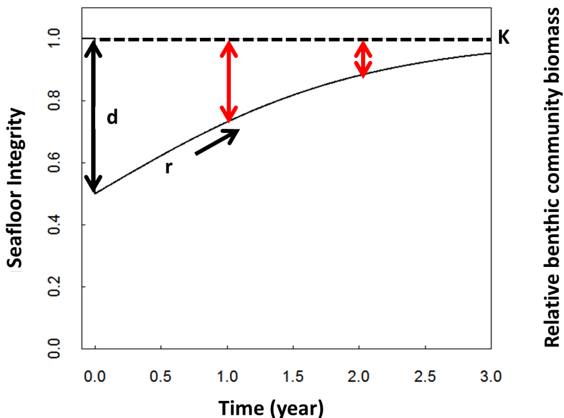
Figure 3.4. Schematic of the parameters: gear-specific Depletion rate ( d ) and habitat-specific Recovery Rate ( r ), which determine the recovery time until K is reached. The benthic invertebrate community biomass is relative to an undisturbed situation (=carrying capacity K , biomass = 1), where impact after 1 and 2 years is indicated by the red arrows.
