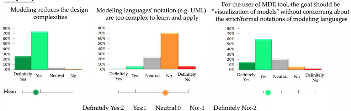
Figure 25. Impacts and implications of MDE in embedded software engineering
