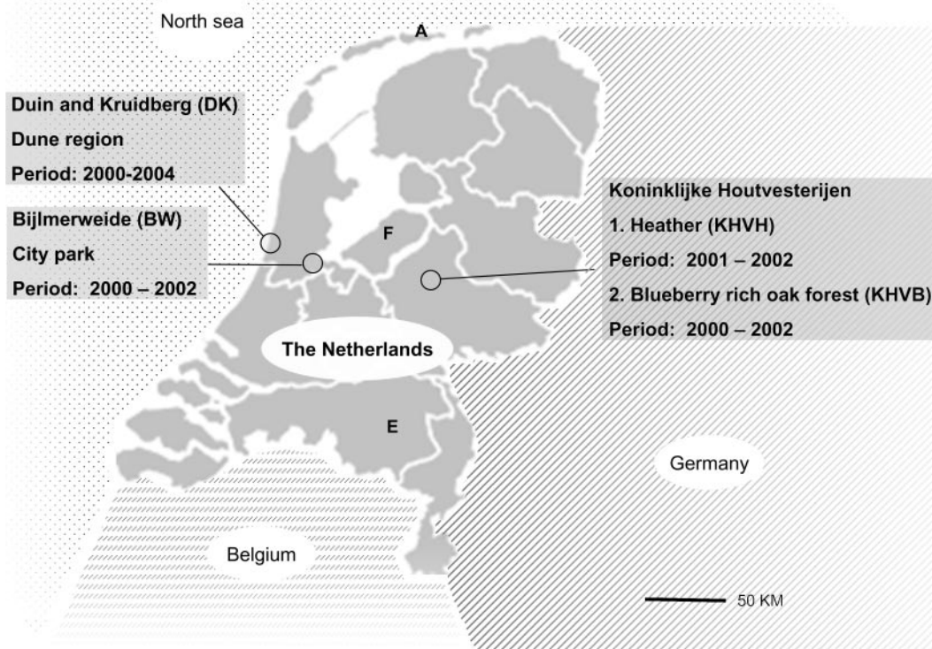
FIG. 1. Locations of the four different habitat areas that were studied. The Netherlands is positioned between the North Sea to the north and west, Belgium to the south, and Germany to the east, and the map shows the four areas that were studied: (i) a dune area, Duin and Kruidberg (DK); (ii) a city park, Bijlmerweide (BW); and the Koninklijke Houtvesterijen, (iii) a blueberry-rich oak forest (KHVB) and (iv) a heather area (KHVH). The years that the ticks were collected in the different areas are indicate. The letters A (Ameland), F (Flevopolder), and E (Eindhoven) indicate the areas previously studied by others (13, 30, 32).
