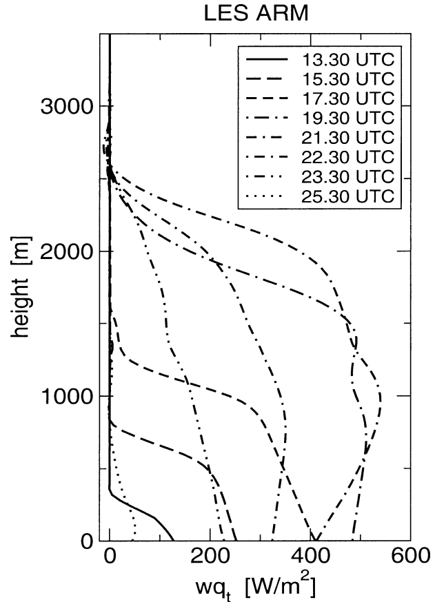
FIG. 4. Vertical profiles of the hourly averaged total moisture flux during the diurnal cycle of the ARM case in LES.
