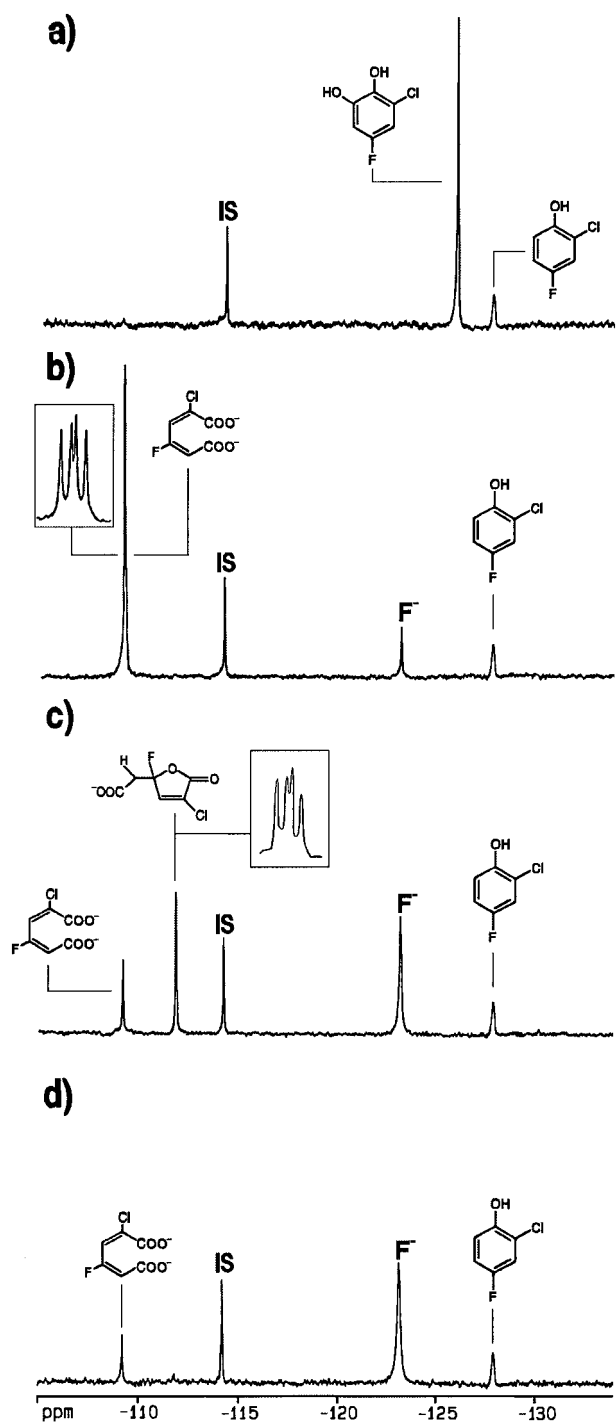
FIG. 1. ^{19}\text{F} NMR analysis of the incubation of 2-chloro-4-fluorophenol with the following: 1.6 \mu\text{M} 2-hydroxybiphenyl mono-oxygenase (a), 1.4 \mu\text{M} ClcA2 (b), 0.5 \mu\text{M} ClcB2 (c), and 1.3 \mu\text{M} ClcF (d).
