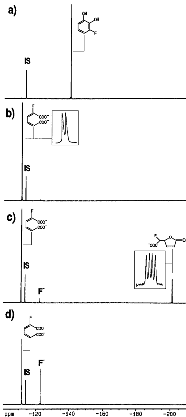
FIG. 2. ^{19}\text{F} NMR analysis of the incubation of 3-fluorocatechol by itself (a) and with the following: 1.4 \mu\text{M} ClcA2 (b), 0.5 \mu\text{M} ClcB2 (c), and 1.3 \mu\text{M} ClcF (d).
