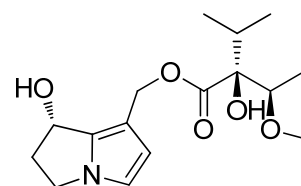
Dehydroheliotrine
