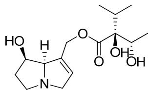
Lycopsamine CAS: 10285-07-1
