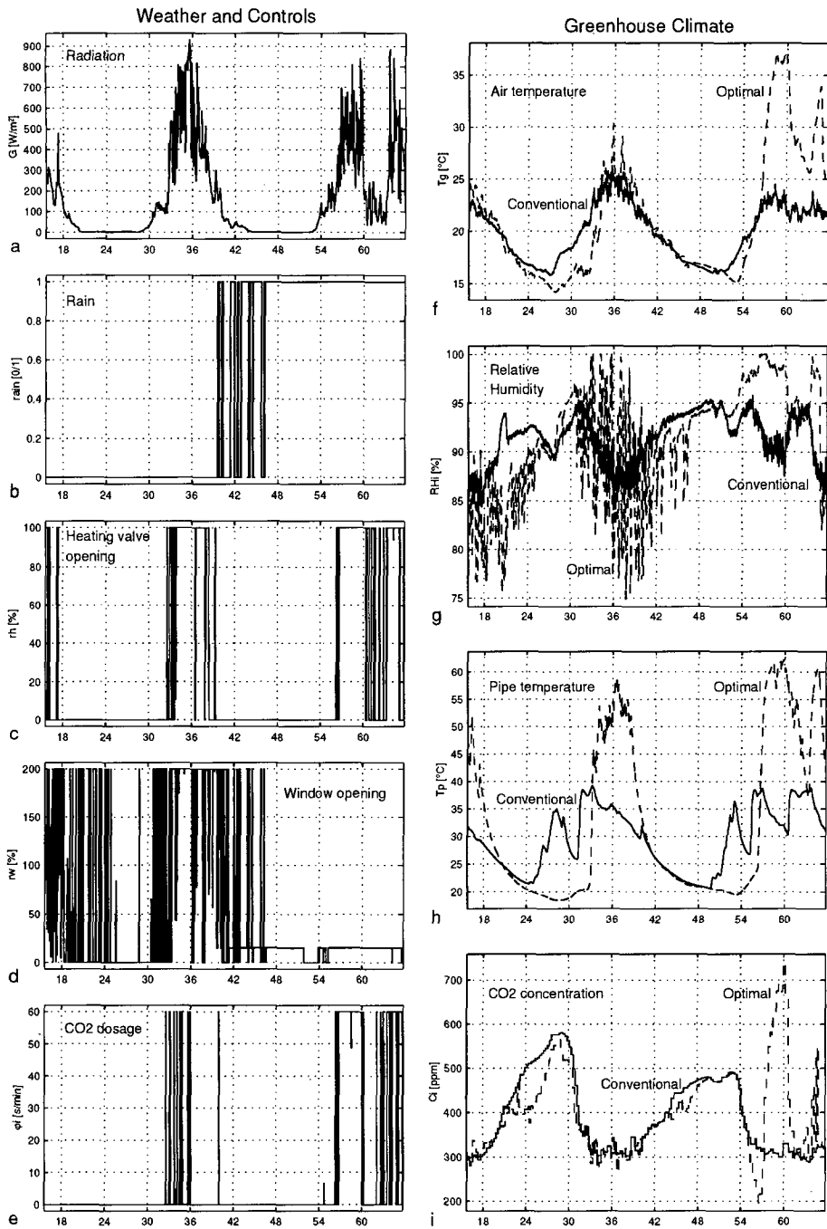
Figure 2 Measured weather, computed optimal controls and measured greenhouse climate for May 19 through May 21 1994.
