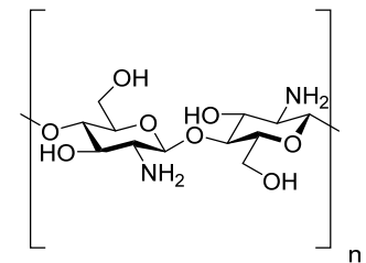
chitosan
