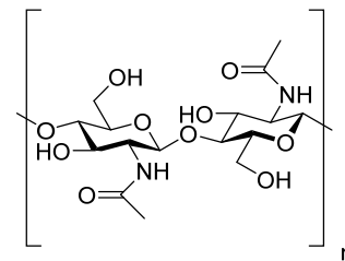
chitine
