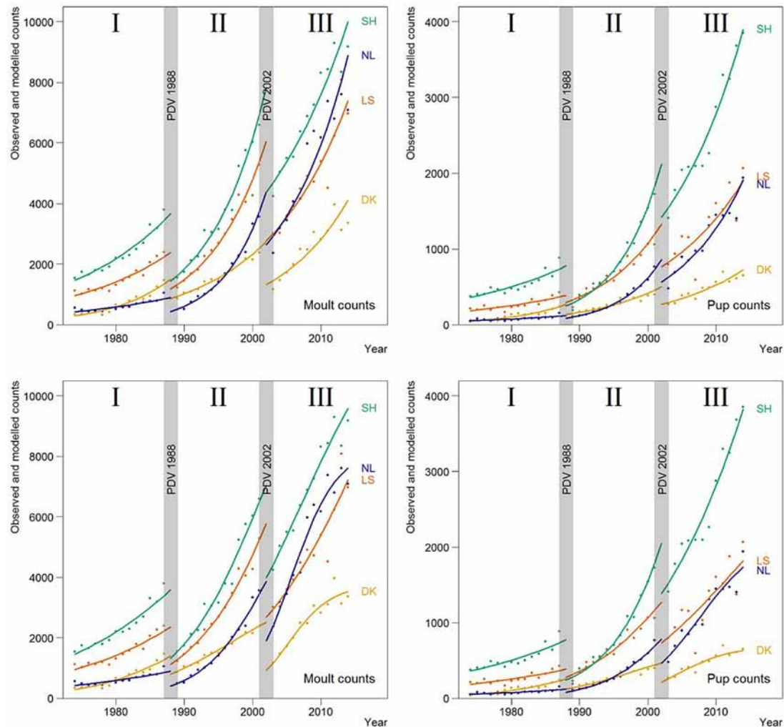
FIGURE 3. RESULTS FOR THE BEST FITTING EXPONENTIAL (TOP) AND DENSITY DEPENDENT MODELS (BOTTOM) FOR THE HARBOUR SEALS IN THE FOUR REGIONS (THE NETHERLANDS (NL), LOWER SAXONY (LS), SCHLESWIG-HOLSTEIN (SH) AND DENMARK (DK)) OF THE WADDEN SEA. THE LINES REPRESENT THE ESTIMATES FOR THE MOULT COUNTS (LEFT) AND PUP COUNTS (RIGHT), AND DOTS THE OBSERVED MAXIMUM COUNTS.
