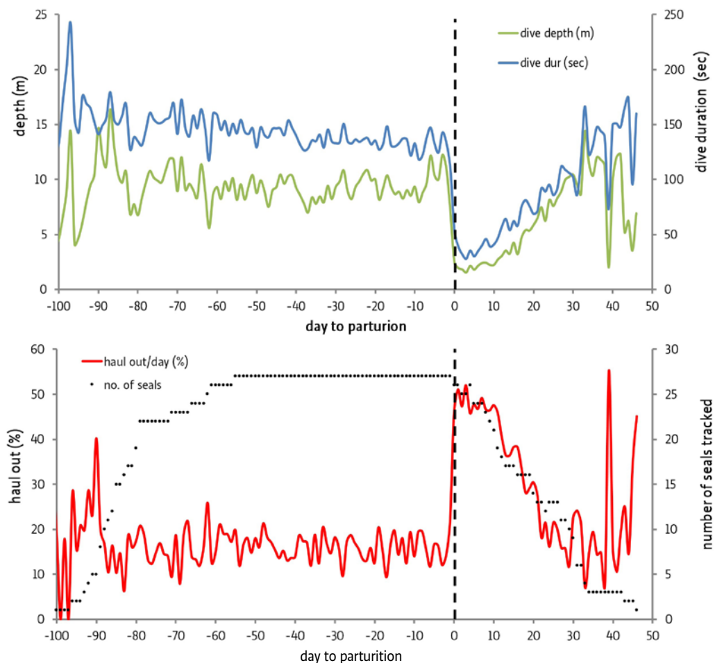
FIGURE 4. FEMALE HARBOUR SEAL BEHAVIOUR IN RELATION TO PRESUMED BIRTH DATE (DASHED BLACK LINE). BOTTOM: AVERAGE HAUL-OUT PERCENTAGE PER DAY (RED) AND NUMBER OF FEMALES PRESUMED BREEDING (BLACK). TOP: AVERAGE MAXIMUM DIVE DEPTH (GREEN) AND MAXIMUM DIVE DURATION (BLUE).
