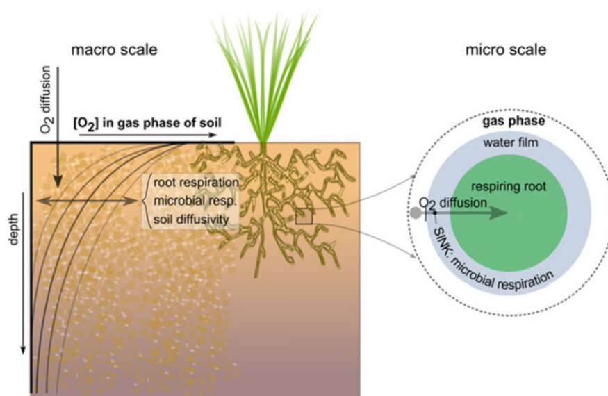
Figure 3.5 Schematization of the oxygen module used to simulate daily respiration reduction. The model combines interacting physiological processes (i.e. root respiration and microbial respiration) and physical processes (i.e. macro-scale and micro-scale oxygen diffusion) (figure from Bartholomeus et al. 2011). Details of equations involved are given in Bartholomeus et al. (2008).
