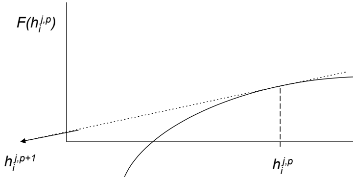
Figure 2.3 Influence of initial estimate on an intermediate solution of a first order approximation based root finding procedure.
