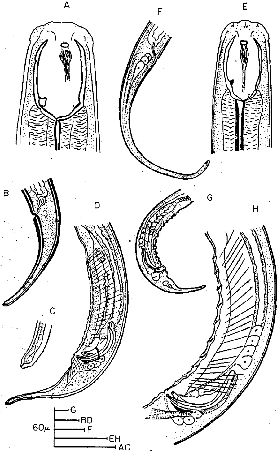
Figure 1. A-D. Iotonchus nayari n. sp. Female: A—anterior end, B—posterior end, C—tail end; Male: D—posterior end. E-H. Iotonchus kherai n. sp. Female: E—anterior end, F—posterior end. Male: G—posterior end, H—spicule and supplements.
