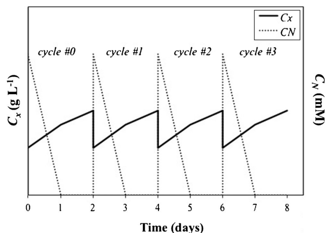
Fig. 1 Schematic representation of a semi-continuous cultivation
