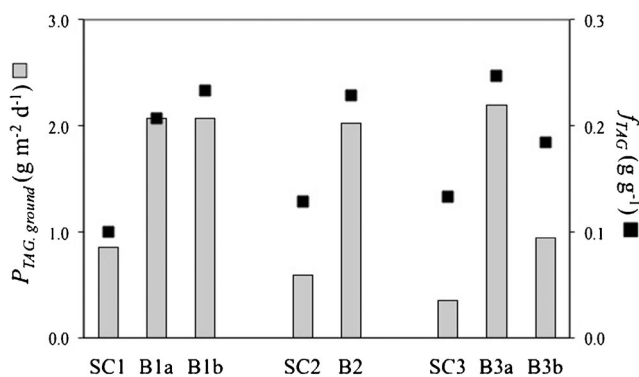
Fig. 5 TAG content ( f_{\text{TAG}} ) and time-averaged ground areal TAG productivity ( P_{\text{TAG, ground}} ) of the outdoor batch (B1a, B1b, B2, B3a, B3b) and semi-continuous (SC1, SC2, SC3) cultivations. For process comparison, P_{\text{TAG, ground}} was calculated over the same period (22, 9 or 26 days) for both operational strategies
