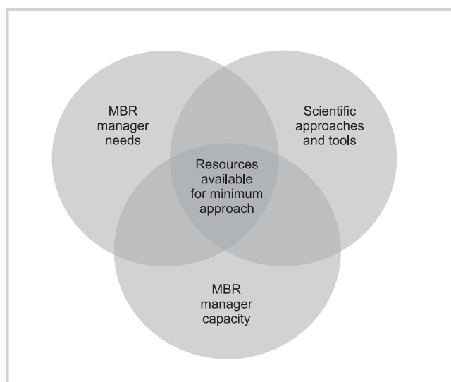
FIGURE 1 Scheme of the set of scientific approaches and tools that are available for predicting the impacts of global change on mountain regions (right), the set of MBRs managers' needs (left), and the set of MBR managers' (or 'local' scientists') capacity to implement such research activities in a given MBR (bottom). Evidently, the contents of the set will vary from one continent to the other, or even from one MBR to the other.
