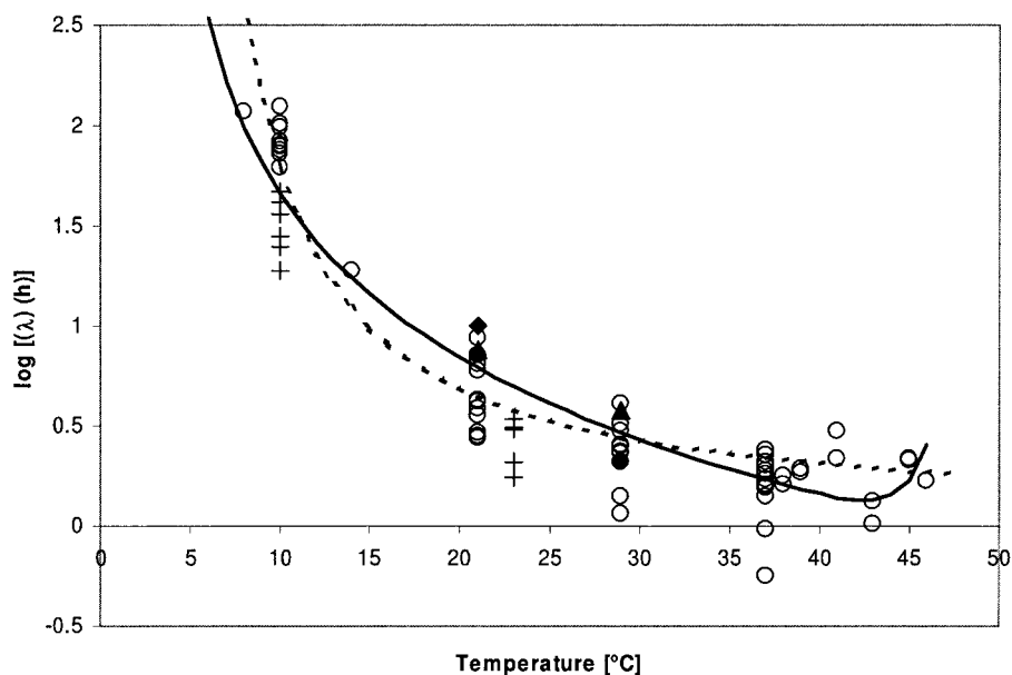
FIG. 4. Log lag times as a function of temperature. ○, ATCC 29544 precultures to various growth phases. Also shown are data for mid-stationary-phase cells of MM9 ●, S94 ◆, and MC10 ▲; lag times at 10 and 23°C as published by Nazarowec-White and Farber (9) (+); and logarithmic transformed lag time data from the present study, modeled with the hyperbolic model (dashed line) and the reciprocal Ratkowsky model (solid line).
