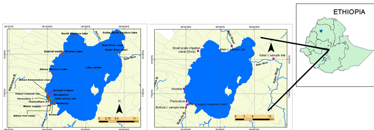
Fig. 1 Physicochemical parameter and pesticide sampling points of Lake Ziway
