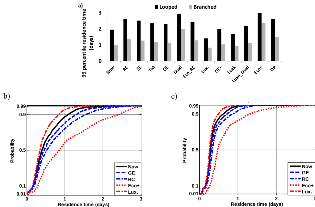
Figure 3-4 a) Variation in the residence time for the 13, (incl now) scenarios. Cumulative distribution of the residence time in the network per meter for five selected scenarios b) looped network and c) branched network.
