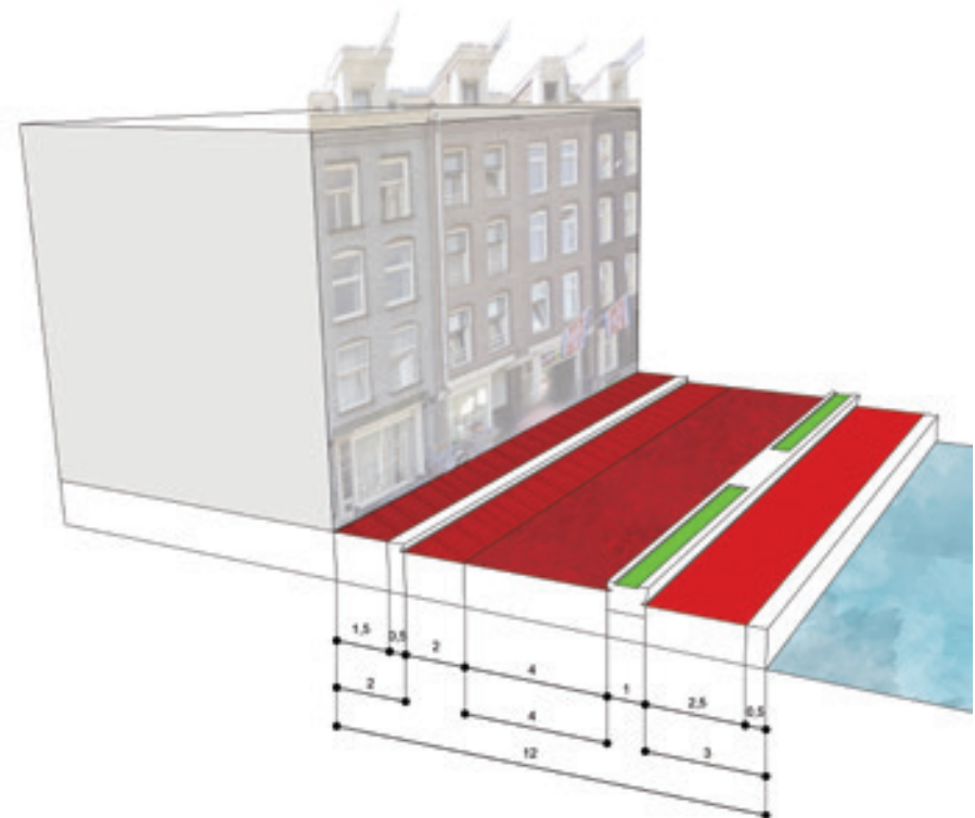
Figure 8.32: 3D section of the average profile
