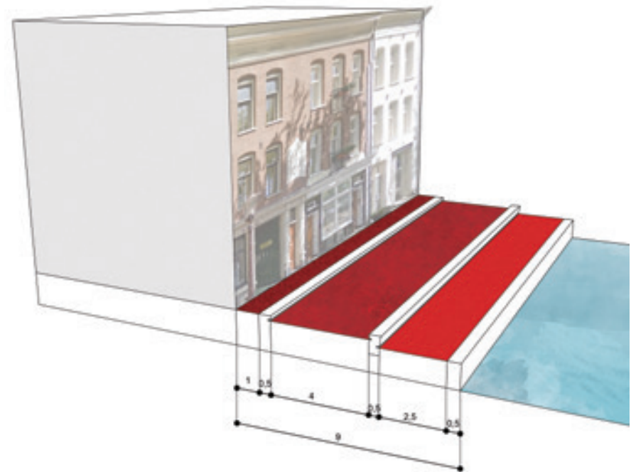
Figure 8.31: 3D section of the smallest profile
