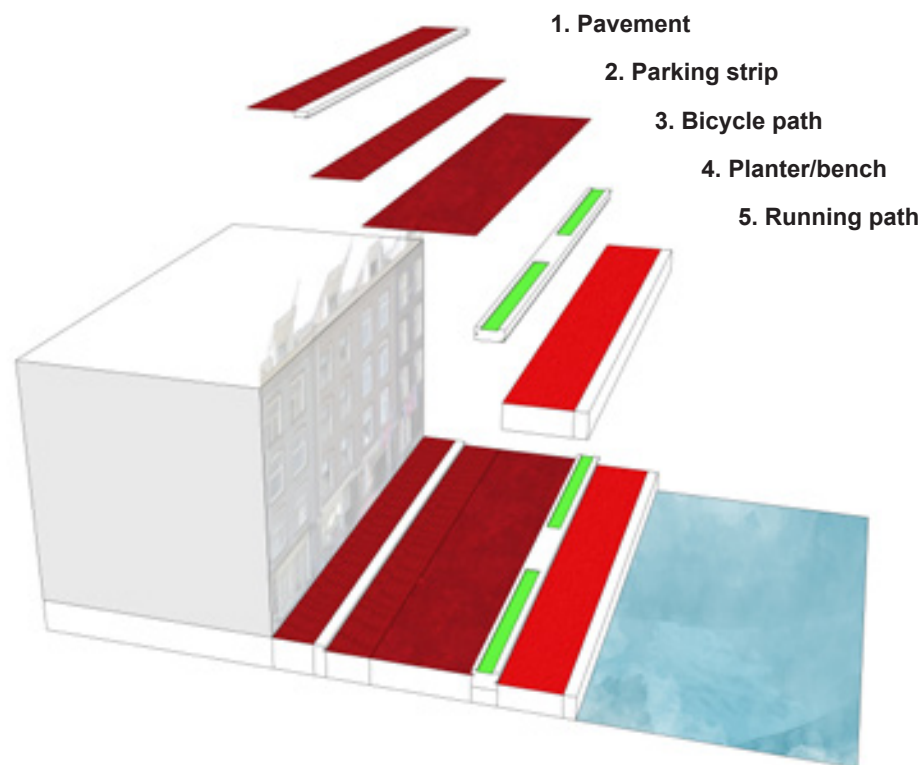
Figure 8.33: Exploded view of broadest profile
