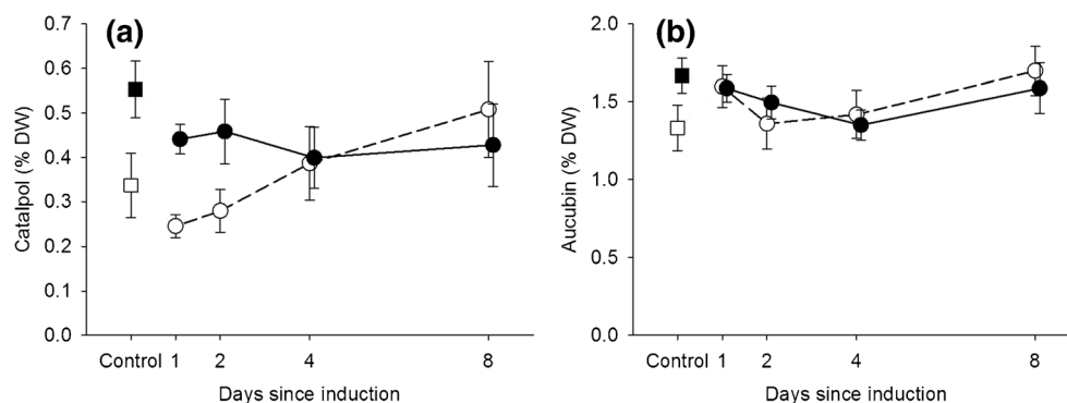
Fig. 3 Mean ( \pm SE) shoot catalpol (a) and aucubin (b) concentration of mycorrhizal (filled symbols, N = 15 ) and non-mycorrhizal (open symbols, N = 13 ) Plantago lanceolata plants that had experienced no herbivory (Control, squares) or a controlled 24 h period of herbivory 1, 2, 4, or 8 d prior to the bioassay (circles). See Table 3 for statistics
