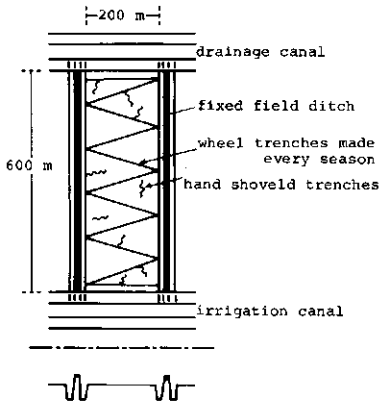
Figure 16. Mechanical trenching with trenchwheel.
