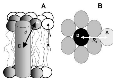
FIGURE 1 Molecular model for the FRET analysis ((A) side view; (B) top view). Protein-lipid organization presents a hexagonal geometry. Donor fluorophore from the mutant protein is located in the center of the bilayer, whereas the acceptors are distributed in the bilayer surface. Two different environments are available for the labeled lipids (acceptors), the annular shell surrounding the protein and the bulk lipid. Energy transfer to acceptors in direct contact with the protein has a rate coefficient dependent on the distance between donor and annular acceptor (Eq. 8). Energy transfer toward acceptors in the bulk lipid is given by Eq. 11 (see text for details).
