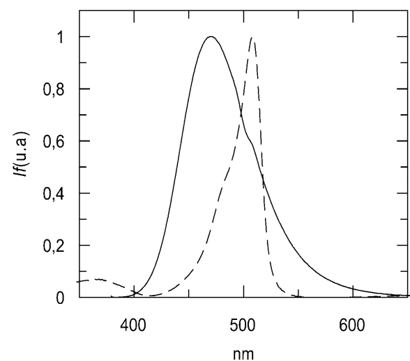
FIGURE 2 Corrected emission spectrum of DCIA-labeled M13 major coat protein (—), and corrected excitation spectrum of NBD-derivatized phospholipid (---).
