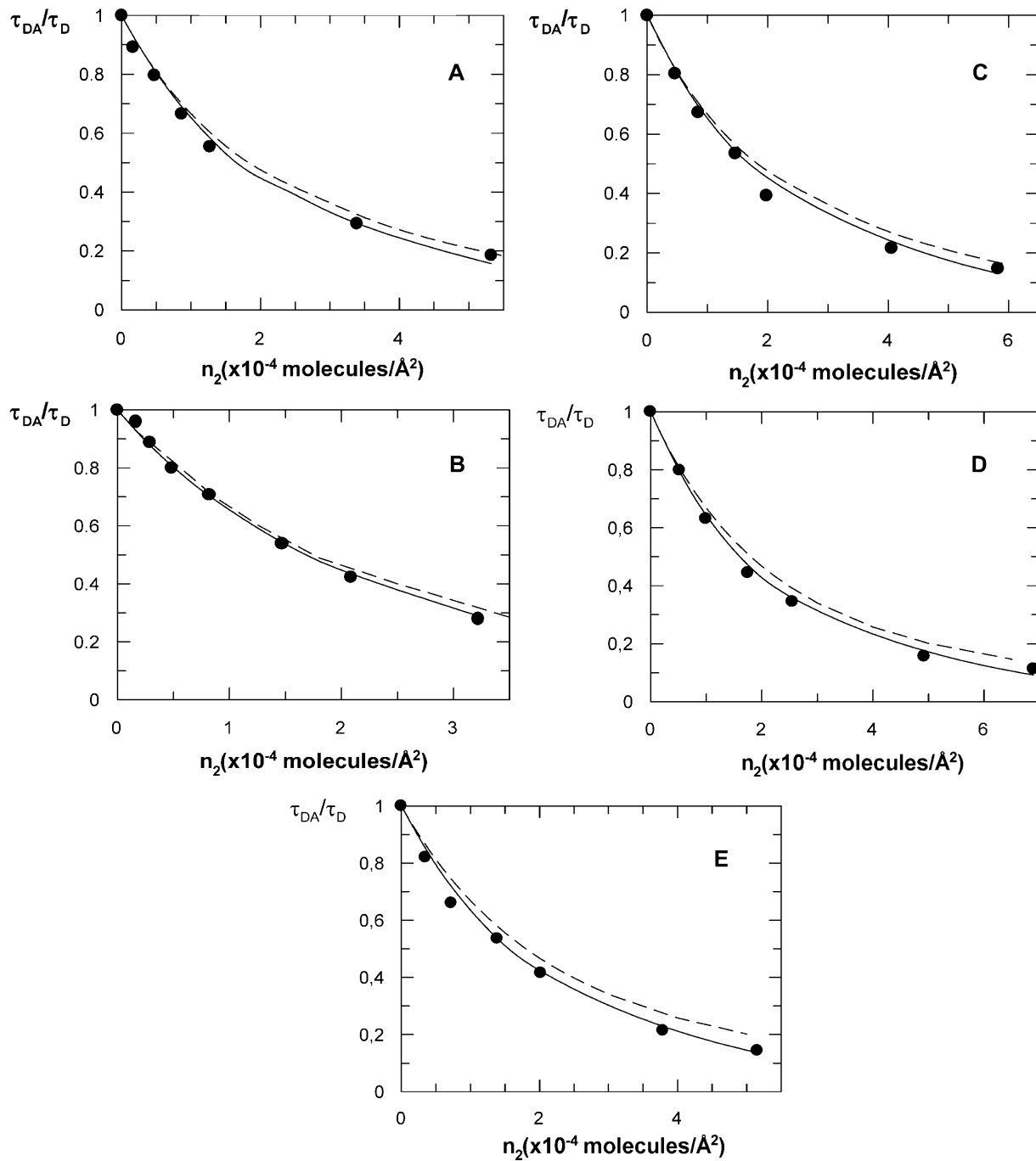
FIGURE 4 Donor (DCIA-labeled protein) fluorescence quenching by energy transfer acceptor (18:1-(12:0-NBD)-PX), where X stands for the different headgroup structures, in pure bilayers of DOPC. (●), Experimental energy transfer efficiencies; (—), theoretical simulations obtained from the annular model for protein-lipid interaction using the fitted K_S ; and (---), simulations for random distribution of acceptors ( K_S = 1.0 ). (A) PC-labeled phospholipid (fitted K_S = 2.0 ); (B) PE-labeled phospholipid (fitted K_S = 2.0 ); (C) PG-labeled phospholipid (fitted K_S = 2.3 ); (D) PS-labeled phospholipid (fitted K_S = 2.7 ); and (E) PA-labeled phospholipid (fitted K_S = 3 ).
