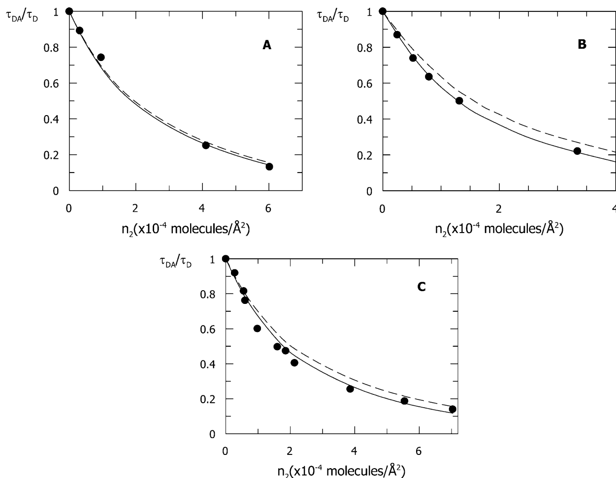
FIGURE 3 Donor (DCIA-labeled protein) fluorescence quenching by energy transfer acceptor ((18:1) 2 -PE-NBD) in pure phosphatidylcholine bilayers with different hydrophobic thickness. (●), Experimental energy transfer efficiencies; (—), theoretical simulations obtained from the annular model for protein-lipid interaction using the fitted K_S ; and (---), simulations for random distribution of acceptors ( K_S = 1.0 ). (A) Labeled protein incorporated in DOPC (fitted K_S = 1.4 ); (B) labeled protein incorporated in DMoPC (fitted K_S = 2.9 ); and (C) labeled protein incorporated in DEuPC (fitted K_S = 2.1 ).
