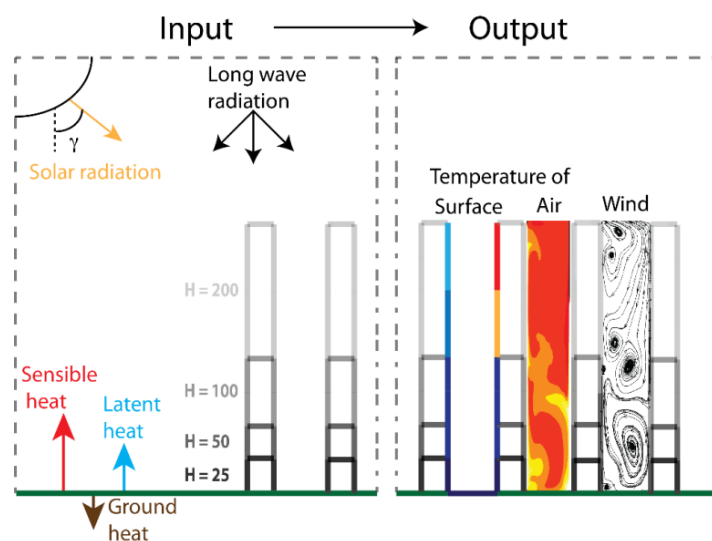
Figure 1.17 Schematic reproduction of the micro scale model developed. The input is on the left, with buildings and accompanying parameters such as height-width ratio, and material properties such as albedo and heat capacity. The various physical properties can be switched on and off independently (ventilation, radiative transfer (short/longwave), etc.). The output is on the right, with surface temperature, air temperature and air currents (Schrijvers et al., 2014).
