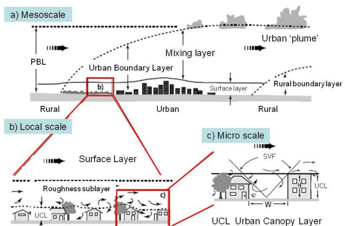
Figure 1.2 The horizontal city scales and the related vertical atmospheric layers. The large arrows indicate the usual direction of the wind; the small arrows show the turbulent air movements. We distinguish three horizontal scales and the related vertical atmospheric layers: 1. Mesoscale (city and surroundings) and the 'Urban Boundary Layer', 2. Local scale (city district) and 'Urban Boundary Layer'/'Urban Canopy Layer', and 3. Micro scale (street, block of housing) and 'Urban Canopy Layer'. PBL-planetary boundary layer, (Source: Oke, 1976).
