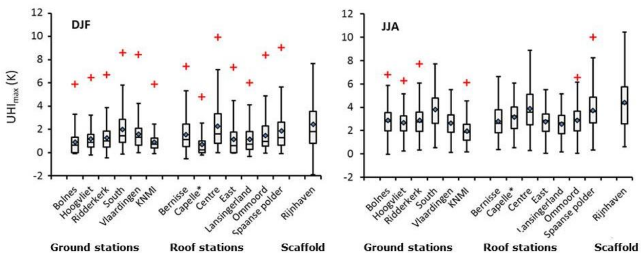
Figure 1.12 Box-whisker plot of UHI_{max} at the measuring locations in the Rotterdam metropolitan area. NB: UHI_{max} is defined as the maximum difference in air temperature between city and surrounding area during a twenty-four hour period. The values have been calculated for the months of June, July and August (JJA) in 2010, 2011 and 2012 and for the months of December, January and February (DJF) in 2009/2010, 2010/2011 and 2011/2012. A distinction was made between rooftop and ground stations (source: Van Hove et al., 2014).
