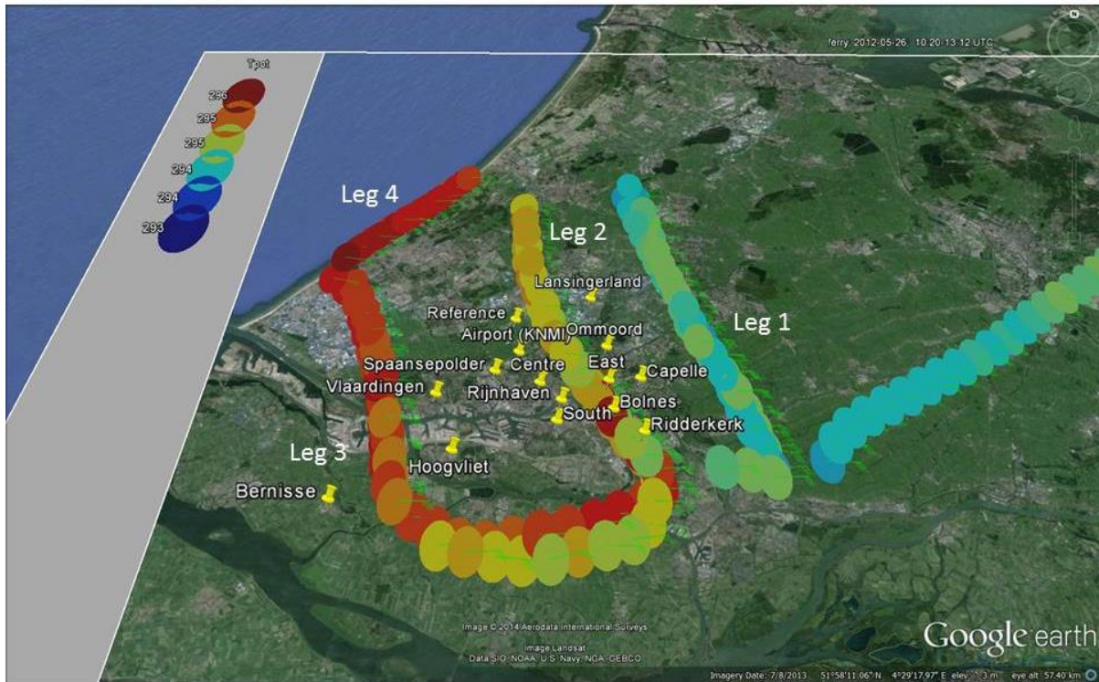
Figure 1.7 Flight paths and measurement results of Lagrangian flights above the southern Randstad at 300 metres on 26 May 2012 between 10:20 and 13:12 UTC (easterly 25-35 kn, clear Q_n \sim 600W m^{-2} , T_{max} 26 \text{ } ^\circ C ). The boundary layer height (for explanation, see Figure 1.2 ) was around 1200 metres at that time. Leg 1 is upwind of the urban area, leg 2 follows a trajectory right across the city (or between the urban areas), leg 3 is downwind. In addition, measurements were taken along the coast (leg 4). The colour of the trajectory corresponds to the surface temperature measured.
