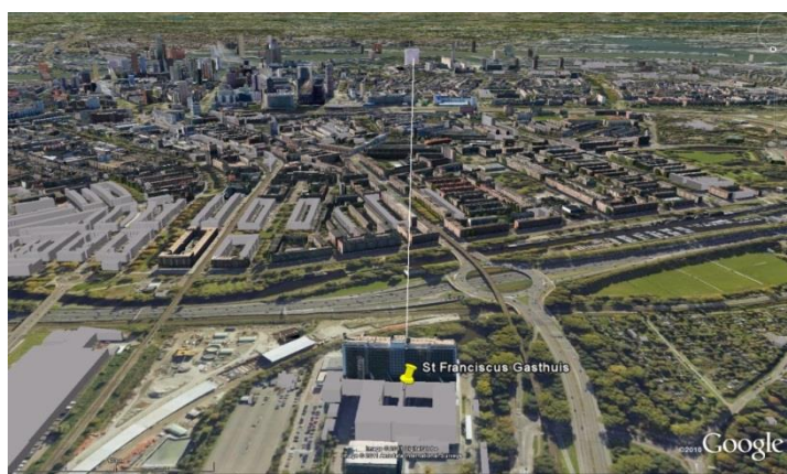
Figure 1.10 Left : Scintillometer path between the Sint Franciscus Gasthuis (Lat/Lon 51.56478/4.27747, elevation 51 metres) and the Erasmus MC (Lat/Lon 51.54632/4.28128, hoogte 77 m) in Rotterdam. The distance between transmitter and receiver is 3451 metres, orientation \sim 180^\circ . Right : set-up for evaporation measurements on top of an apartment complex on the Ingenieur J. P. Van Muijlwijkstraat in Arnhem (51°59'4.97"N, 5°55'5.73"E) http://www.climatexchange.nl/sites/arnhem/index.htm . The measuring system consists of a 3D ultrasonic anemometer (Gill R3-50) in combination with a fast open-path infrared gas analyzer (Li-Cor LI-7500) attached to the top of a 4-metre-high mast.
