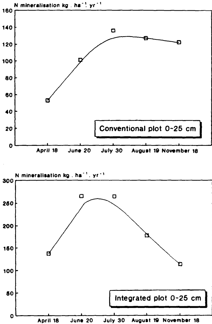
Fig. 4. Potential nitrogen mineralization rates during 1986. Mind the different scales of the Y-axes.
