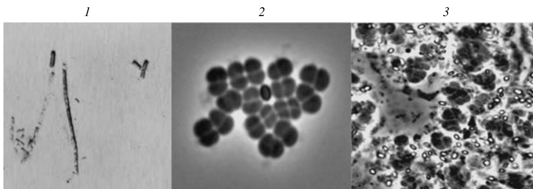
Fig. 2. Cell morphotype at various biodegradation stages: (1) chains of heteromorphous rods packed in a common mucous envelope; (2) Methanosarcina -like cells; (3) methanogenic grains.
