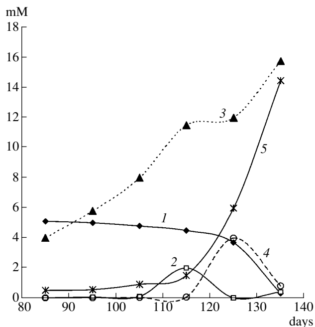
Fig. 1. Degradation of 2-ABA by a methanogenic association: (1) 2-ABA, (2) benzoate, (3) ammonia, (4) acetate, (5) methane.
