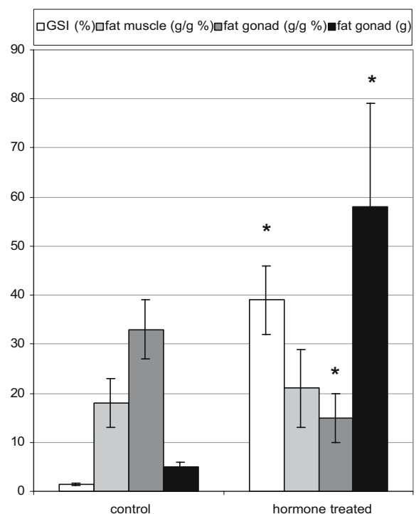
Fig. 1 GSI (relative gonad weight), relative fat content in muscle and gonad (g fat/g tissue \times 100%) and total fat in gonad (g/kg eel) in control and hormone-treated eels. Highly significant differences ( P<0.001 ) between groups are indicated by an asterisk
