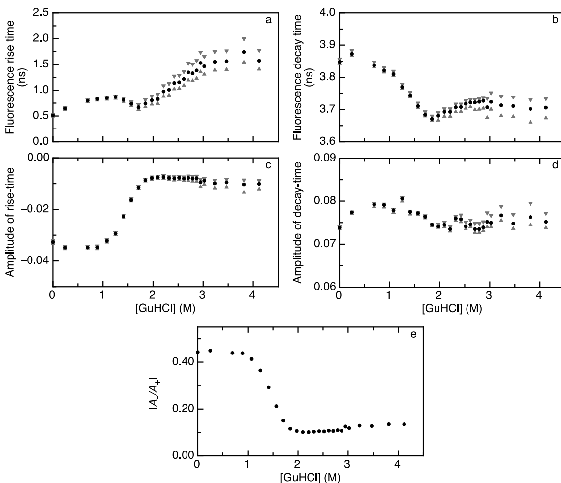
Figure 2. Denaturant-dependencies of rise and decay times of acceptor fluorescence upon donor excitation track folding of apoflavodoxin labeled with A488 (donor) and A568 (acceptor). In all panels, black dots represent fitted values and grey triangles represent confidence limits. (a) The rise time of acceptor fluorescence and (b) decay time of acceptor fluorescence reveal the biphasic dependencies on GuHCl; (c) The amplitude of the acceptor fluorescence rise time ( A_- ) changes in a monophasic manner as a function of GuHCl; (d) The amplitude of acceptor fluorescence decay ( A_+ ) is virtually constant as a function of denaturant concentration; and (e) The absolute ratio of the amplitudes of fluorescence rise and decay time ( |A_-/A_+| ) shows a monophasic dependence on denaturant concentration.
