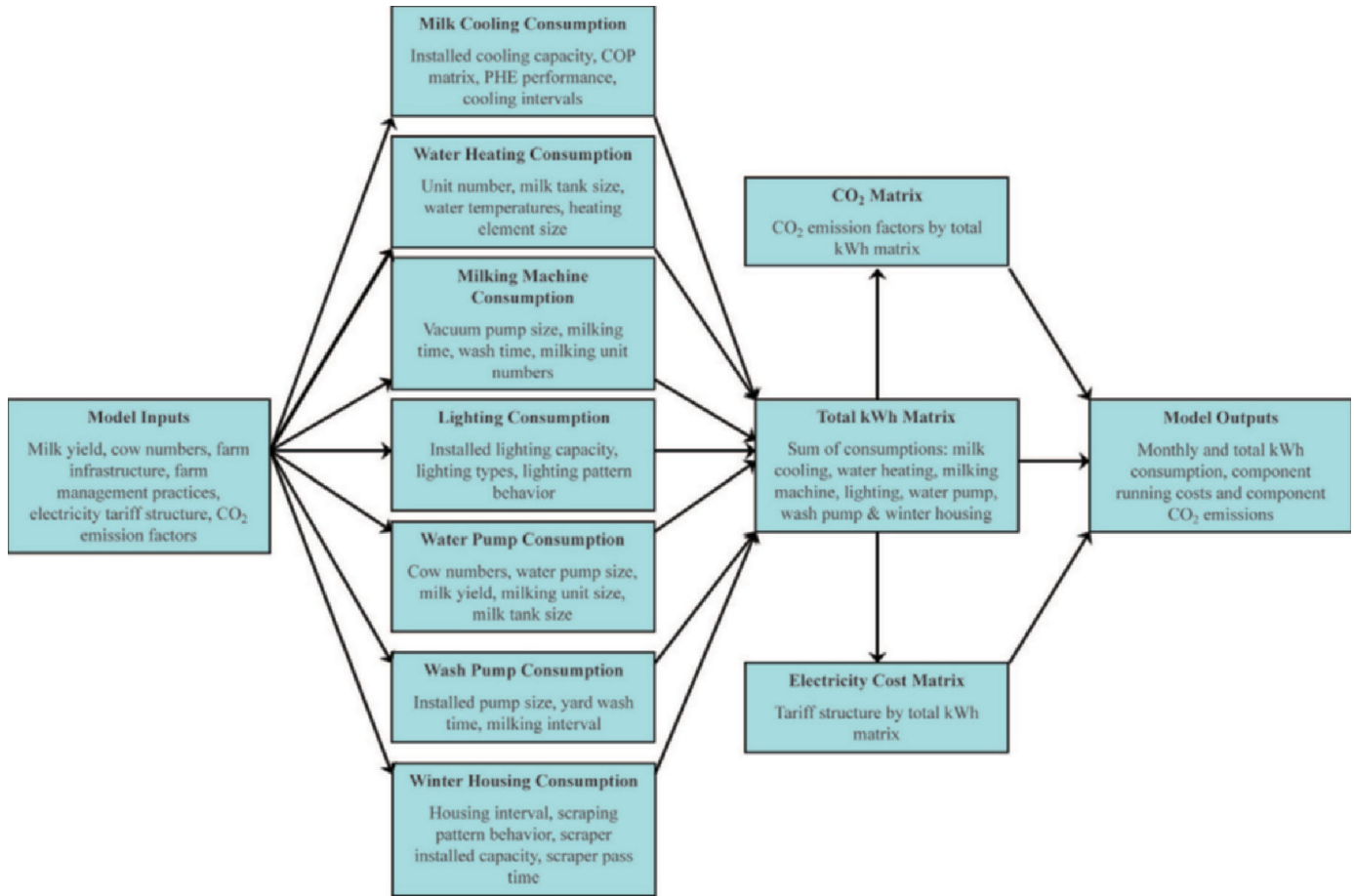
Figure 1. Schematic of milk production electricity consumption model showing the 4 primary sections, illustrated from left to right: (1) inputs, (2) consumption matrix calculations for the 7 main infrastructural systems, (3) consumption summing and tariff application, and (4) outputs. COP = coefficient of performance; PHE = plate heat exchanger. Color version available in the online PDF.
