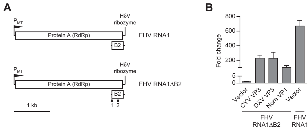
Figure 5. CYV and DXV VP3 rescue replication of a B2-deficient FHV RNA1 replicon. (A) Schematic representations of FHV RNA1 and FHV RNA1ΔB2. The replicons are launched from a copper-inducible metallothionein promoter ( P_{MT} ). Their 3' end is defined by a Hepatitis delta virus (HδV) ribozyme. Mutations in the B2 coding sequence are indicated by arrow heads. Mutation 1 (T2739C; with respect to the FHV RNA1 sequence; GenBank accession number: X77156.1) disrupts the AUG start codon and mutation 2 (C2910A) introduces a premature UAA stop codon. RdRp, RNA-dependent RNA polymerase (B) FHV RNA1 replicon assay in S2 cells. The FHV RNA1ΔB2 replicon was transfected into the cells together with an empty vector control (Vector) or a plasmid encoding either CYV or DXV VP3. An expression plasmid for Nora virus VP1 (Nora VP1) was used as positive control. The wild-type FHV RNA1 replicon was transfected together with the empty vector control to indicate wild-type replication levels. FHV RNA1 replication levels were quantified by qPCR and normalized to RpL32. The data are presented as fold change relative to FHV RNA1ΔB2 co-transfected with the empty vector control. Bars and error bars in (B) represent the mean and standard deviation of three independent samples.
