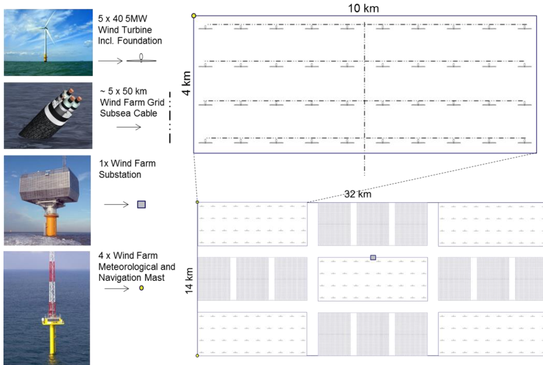
Figure 7-7. Wind farm including auxiliary systems.
