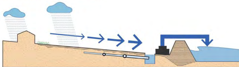
Pipe - Pump - Drain
