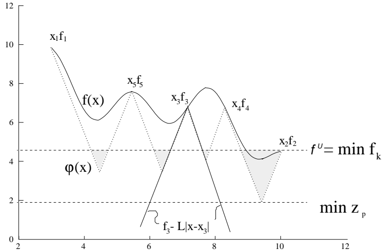
Figure 4: Piyavskii-Shubert algorithm
