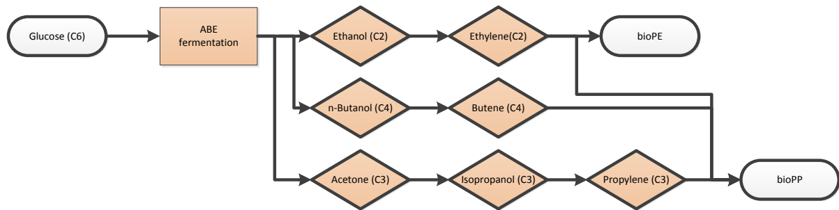
Fig.14 – Glucose conversion by ABE fermentation for polyolefin production
