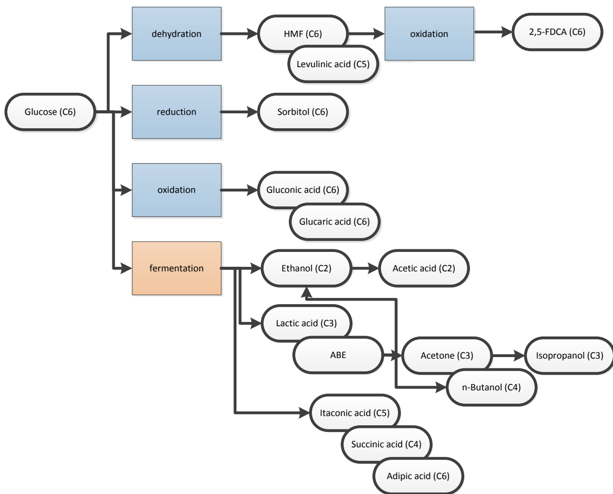
Fig.8 Sugar (hexose, C6) as platform commodity as feedstock for conversion processes to key 'green' chemicals by chemical and enzymatic processes
