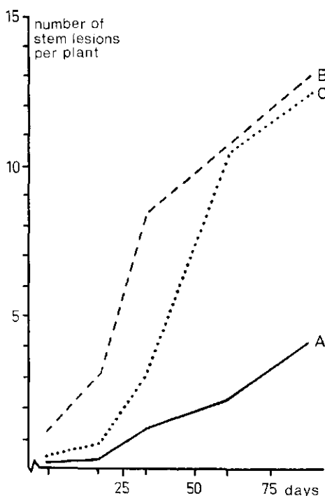
Fig. 2. Effect of the method of deleafing on the occurrence of stem lesions, caused by B. cinerea . Deleafing was done at the "normal time".
