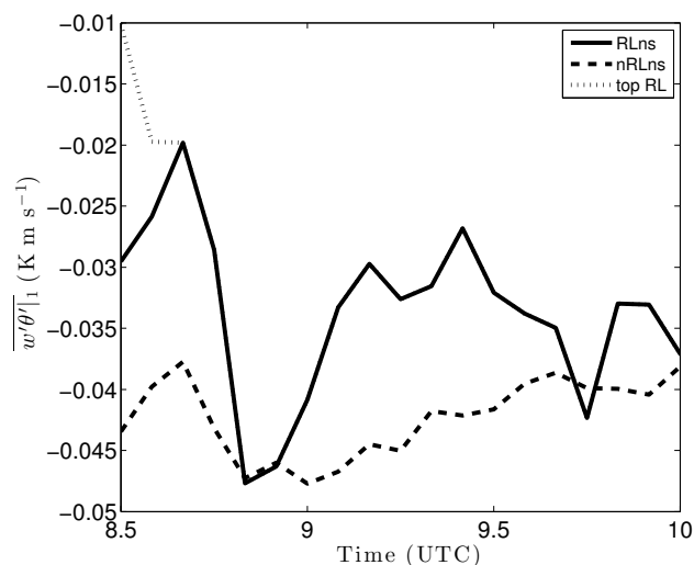
Fig. 6. Temporal evolution during the morning of the entrainment heat flux for the RLns (solid line), the entrainment heat flux at the top of the RL (pointed line) and nRLns (dashed line) DALES numerical experiments.
