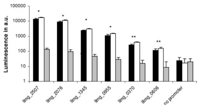
FIG. 2. Effect of addition of riboflavin or FMN on luminescence signals of stationary-phase cells of L. lactis MG5267 with various luciferase expression levels. Luciferase activity was measured 3.5 h after cultures entered the stationary phase. The black bars show measurements performed in buffer supplemented with 10 mg/liter riboflavin. White bars show measurements in buffer supplemented with 10 mg/liter FMN. Gray bars show measurements in buffer only. Each bar represents the average value of four biological replicates (error bars show standard deviations). *, P < 0.001 ; **, P < 0.002 (pairwise t test). The experiment was repeated four times with similar results. The names of the samples refer to the promoter sequences upstream of the luciferase genes as annotated in L. lactis MG1363 (18). a.u., arbitrary units.
