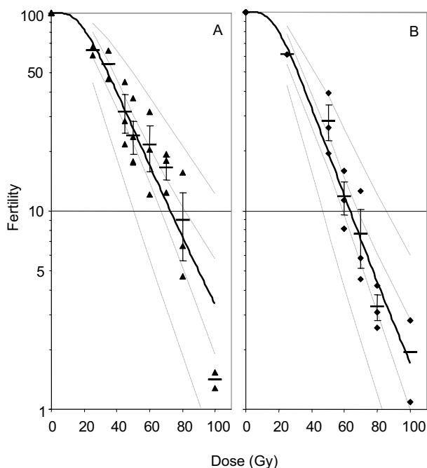
Figure 3 Regression line (± 95% CI for mean and individual values) for fertility versus irradiation dose (Gy) for male An. arabiensis pupae (A) and adults (B). Symbols indicate observed individual values. Means (± SE, if n>2) are indicated by a horizontal line.
