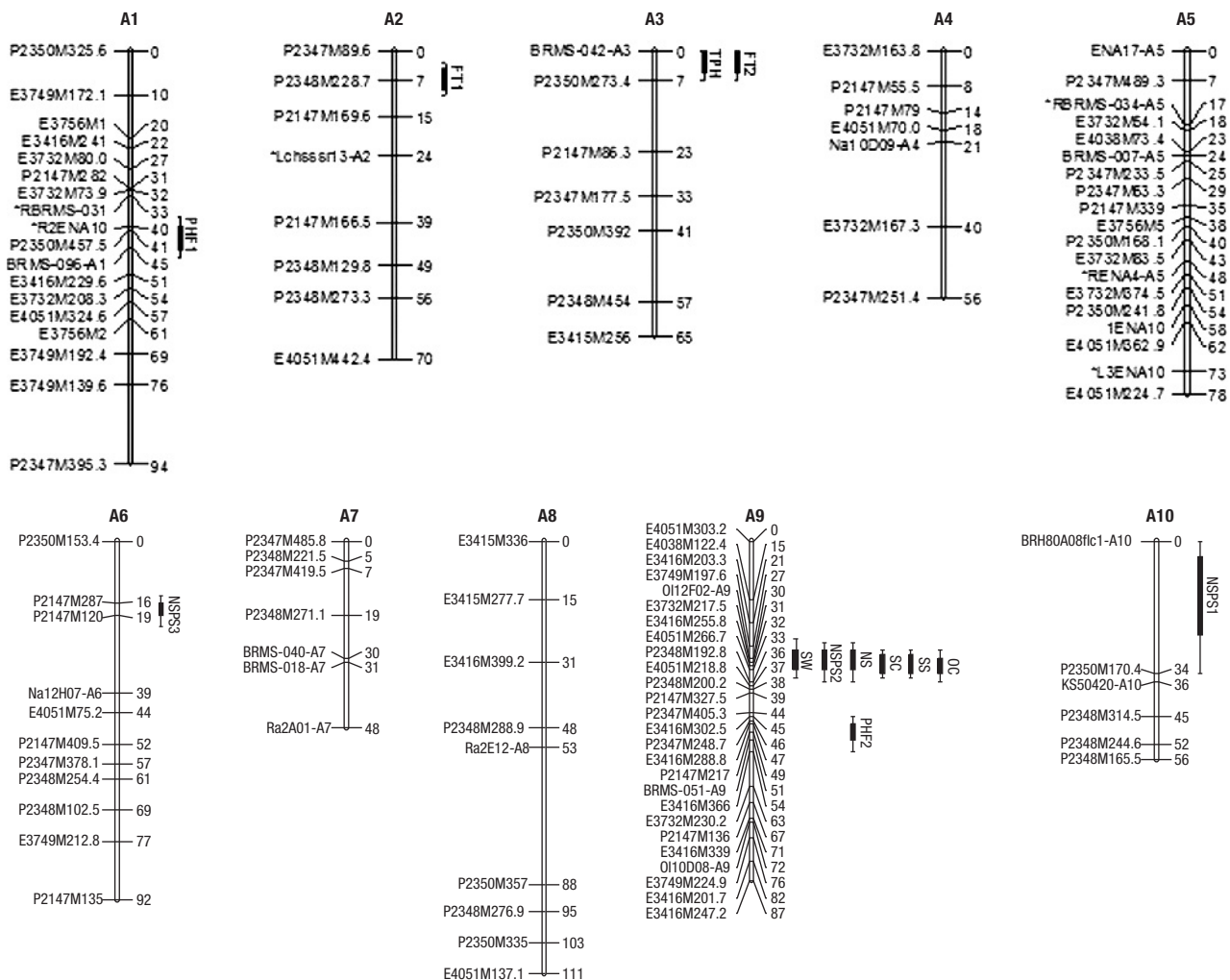
Figure 1. Linkage map of the L58 × R-o-18 F 2 population including ten linkage groups (A1-A10), showing the positions of 97 AFLPs, starting with P ( Pst I) or E ( Eco RI), and 21 SSRs. QTL are indicated with boxes and whiskers representing 1- and 2-LOD confidence intervals (95%) respectively. Skewed SSR markers in A1, A2 and A5 are indicated with * and letters L or R to show if these markers are coming from L58 or R-o-18 respectively.
